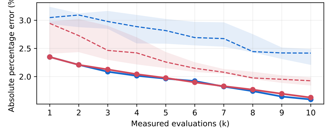
C Score reconstruction — MEDAPE
