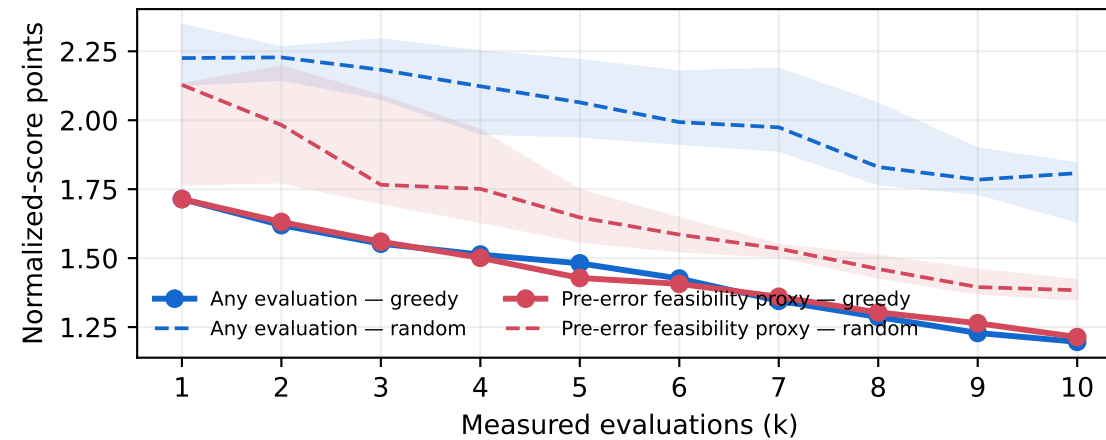
B Score reconstruction — MEDAE
