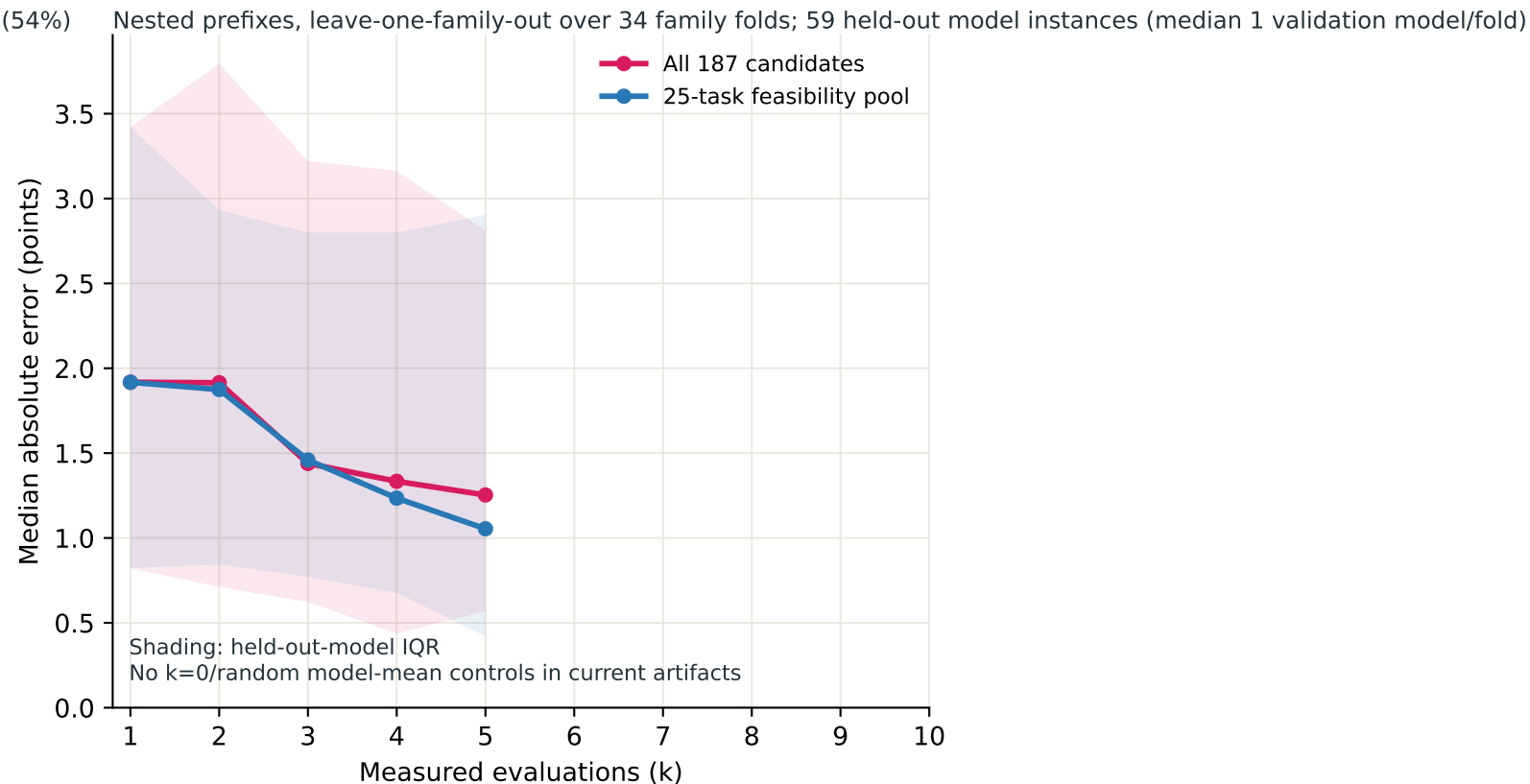
B Error predicting mean reported score
