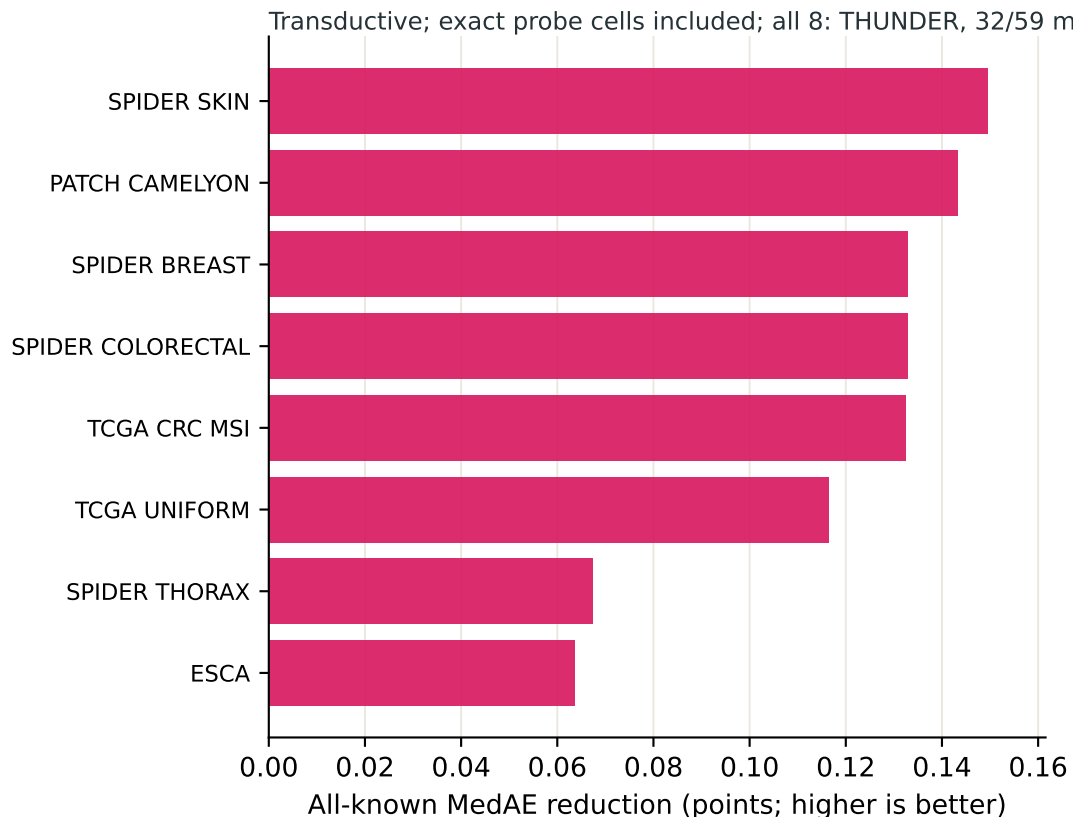
A Retrospective single-task utility
