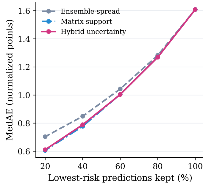
A Risk-coverage
