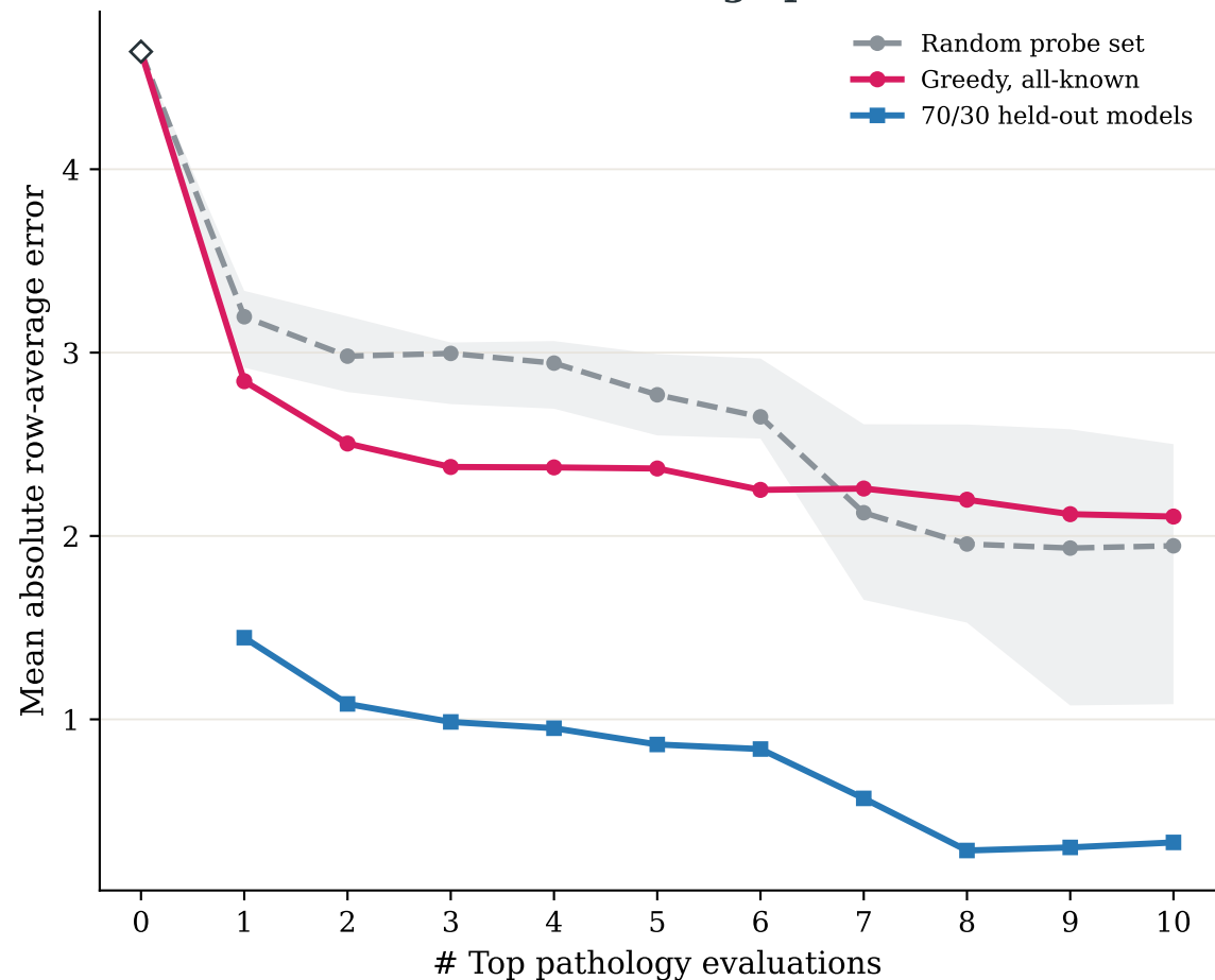
Literal model-average prediction
