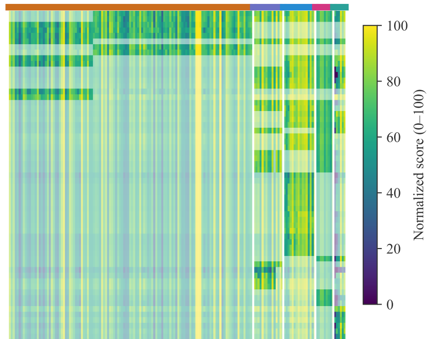
Completed matrix (latent interaction rank 1)
