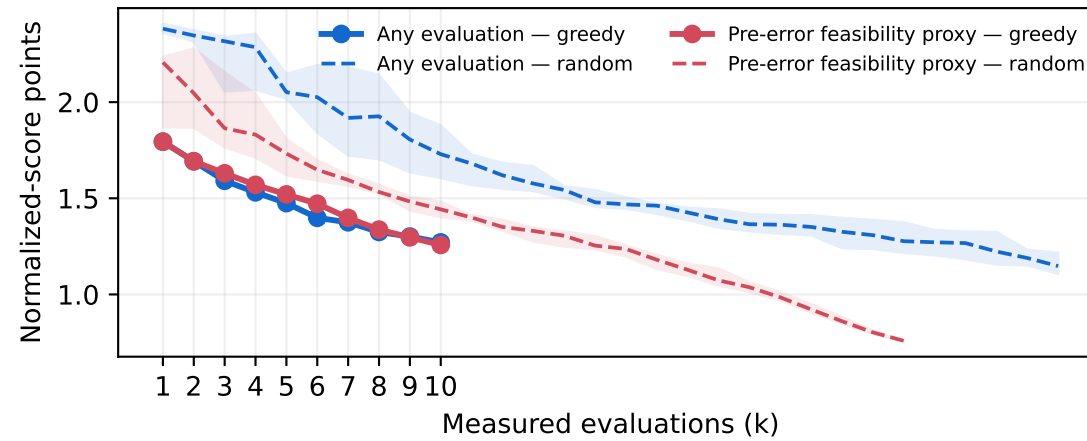
B Score reconstruction — MEDAE
