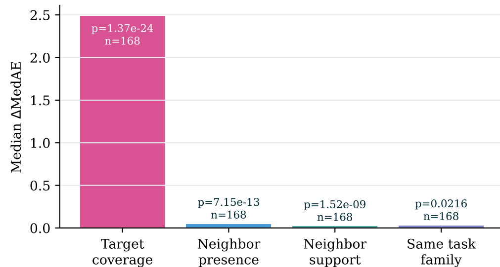
D Paired evidence interventions
