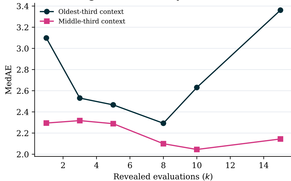
D Training-anchor recency
