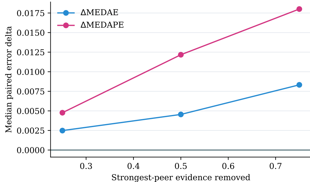
B Peer-support dose response
