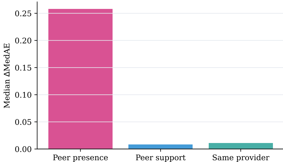
A Peer-evidence ablations
