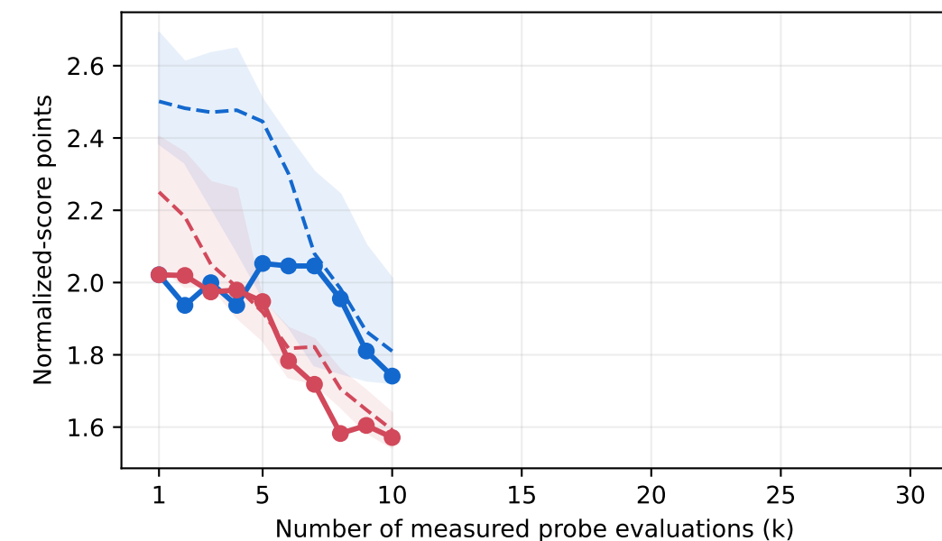
Held-out models — MEDAE
