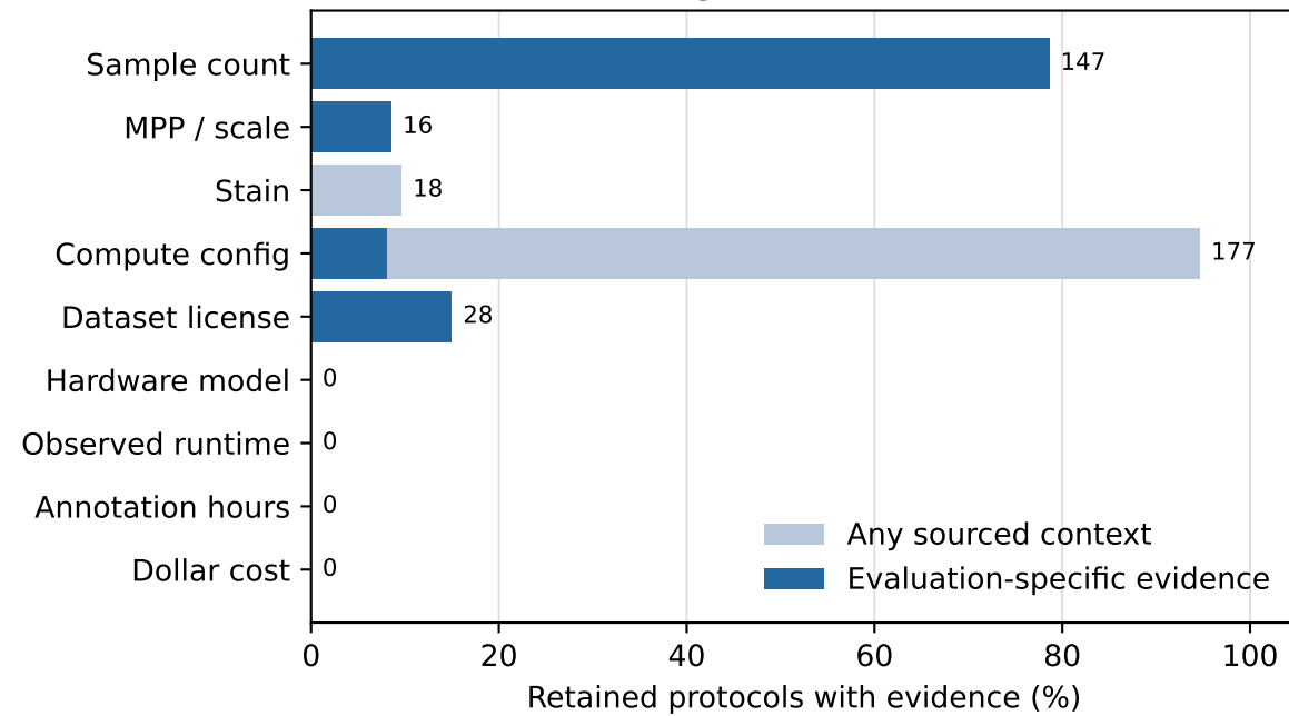
A. Evidence coverage (n=187)
