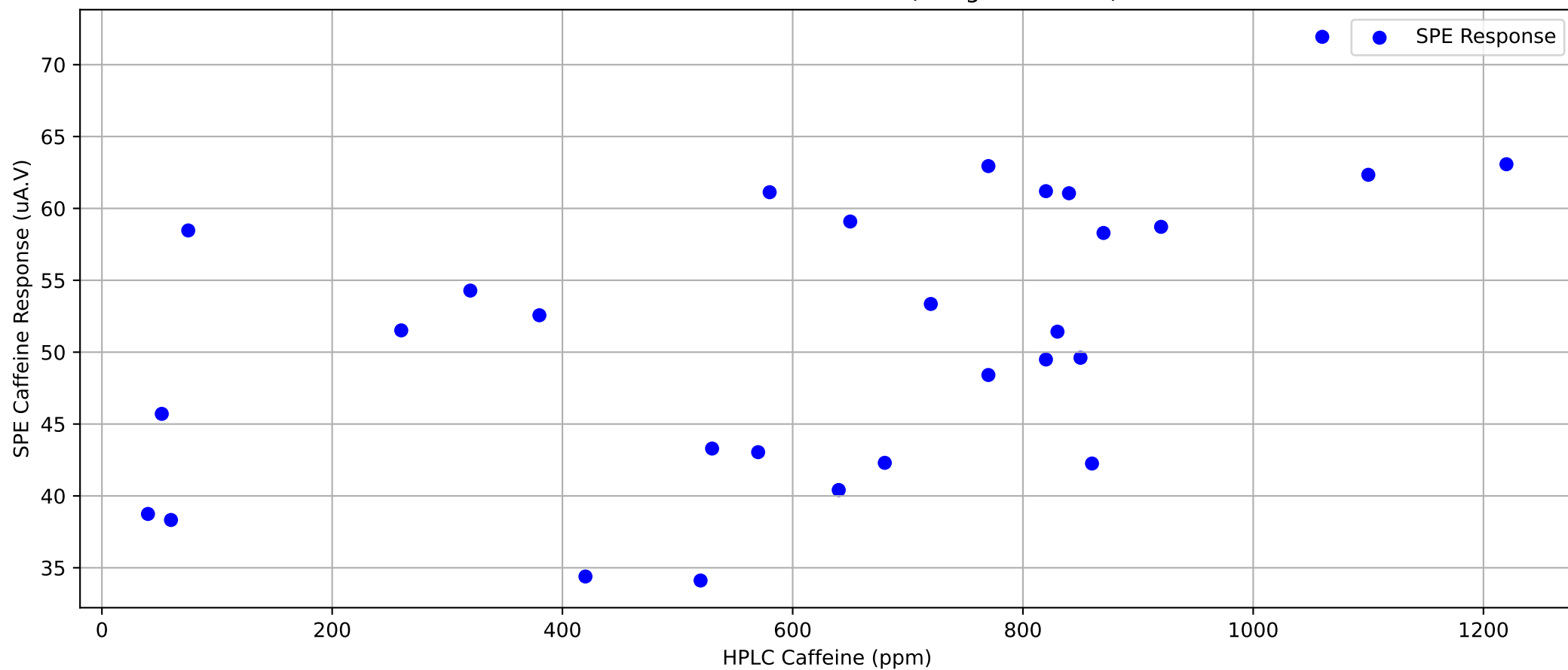
HPLC Caffeine vs SPE Caffeine (Integral Method)
