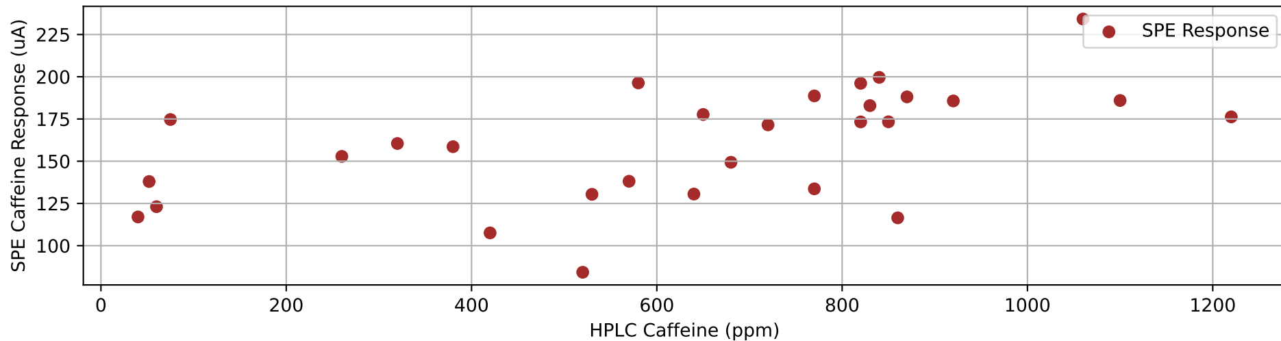
HPLC Caffeine vs SPE Caffeine (Peak Method)
