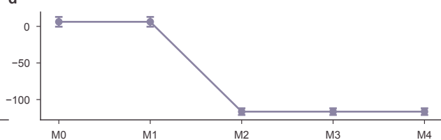
d Loss-CVaR
