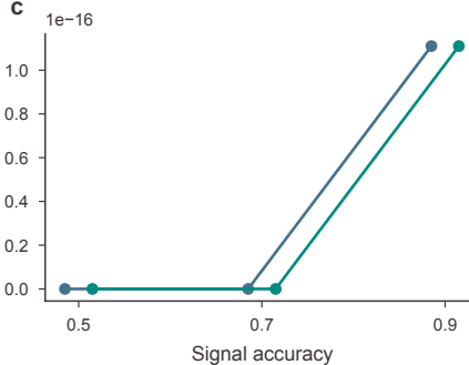
c Dominated option · unrelated
