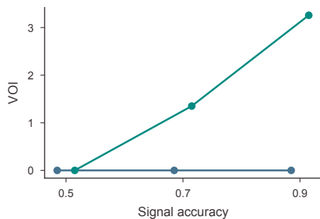
e Registered interaction estimates
