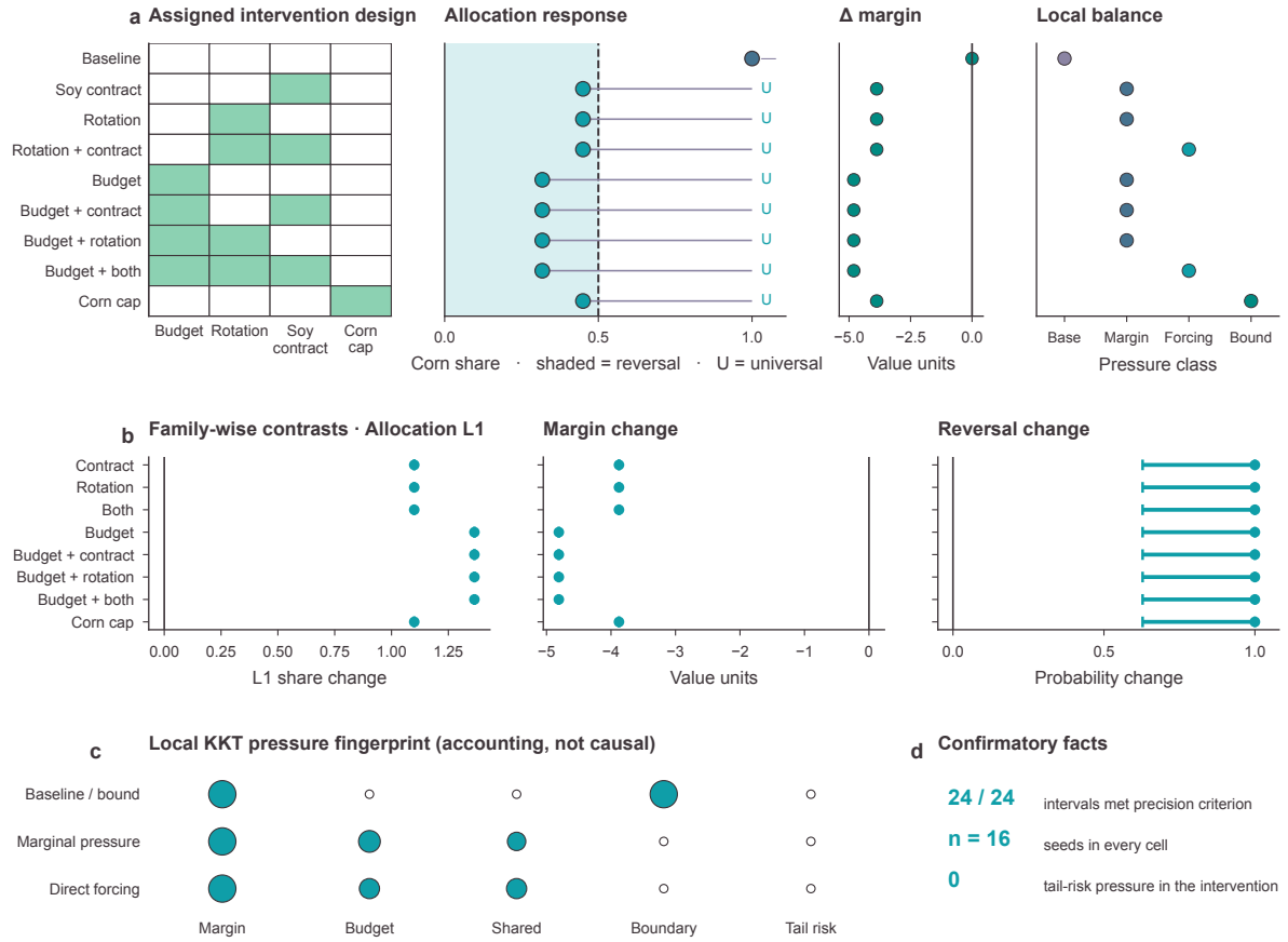
Figure 4: Assigned operational interventions identify reversal. The aligned top row links the factorial intervention design to selected allocation, universal-reversal classification, margin change and local pressure class. The lower panels report three families of contrasts, the KKT pressure fingerprint and confirmatory facts. Each cell has n = 16 and all 24/24 intervals meet the pre-specified precision criterion.
