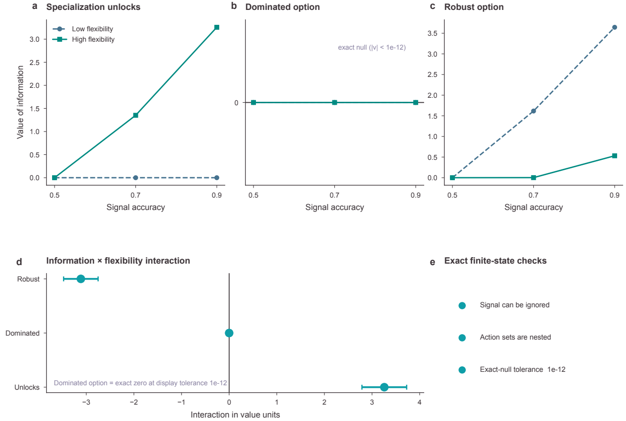
Figure 5: Information and action-set flexibility can complement, substitute or be unrelated. The display reports three pre-specified archetypes, their interaction intervals and exact finite-state checks. For the dominated option, values with absolute magnitude below 10^{-12} are displayed as exact zero; the source values are unchanged. All three family-wise intervals meet the pre-specified precision criterion.
