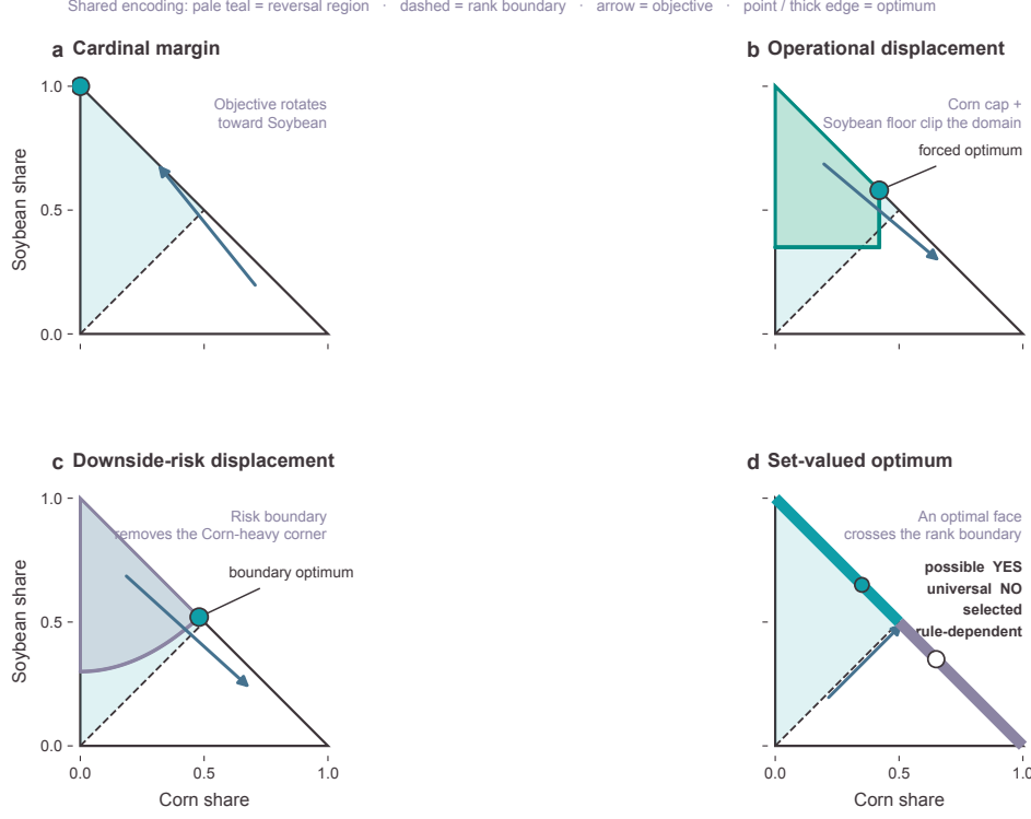
Figure 2: A four-mechanism atlas on shared coordinates. Each panel uses the same Corn–Soybean simplex and rank boundary but distinguishes the feasible region, objective direction and optimal point or face. Cardinal margins rotate the objective; operational restrictions clip the domain; downside risk truncates a preferred corner; and a set-valued optimum crosses the boundary. These are exact analytic constructions, not empirical estimates.
