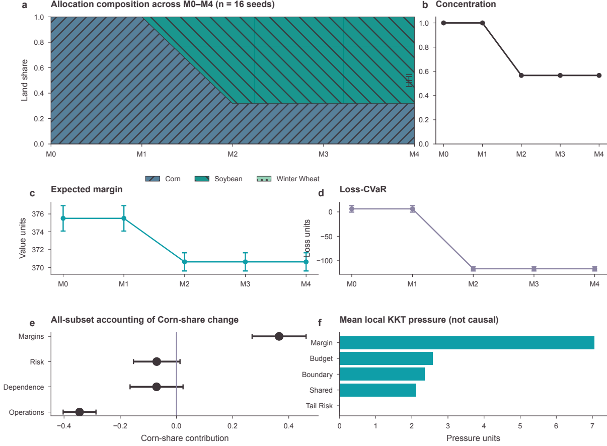
Figure 3: Nested allocation and mechanism decomposition. The staged path reports crop allocation, expected margin and loss-CVaR in native units, all-subset Shapley contributions and signed KKT pressures from the operational intervention. Intervals summarize repeated simulations; pressure terms are local accounting identities rather than causal acreage effects.
