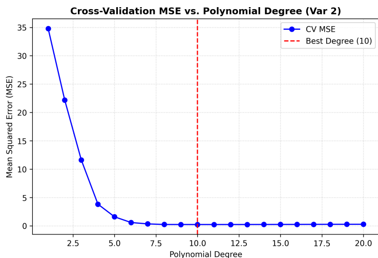
Figure 3: Polynomial degree vs MSE for var2
