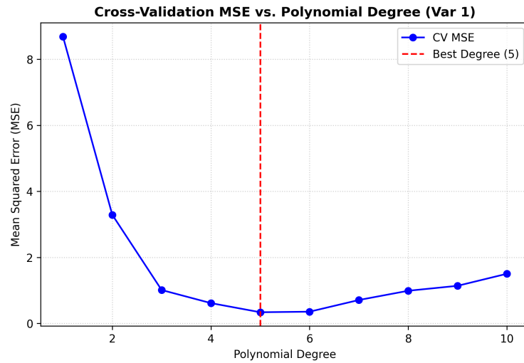
Figure 1: Polynomial degree vs MSE for var1
