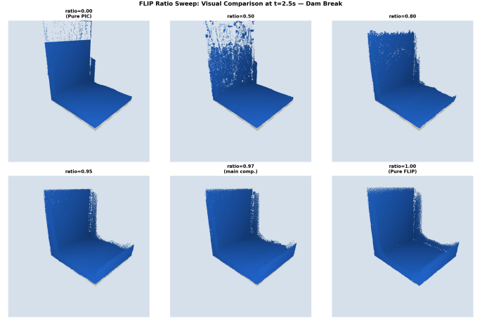
Fig. 9. FLIP ratio sweep visual comparison at t = 2.5s for the dam-break scene. Pure PIC shows a barely propagating wave; pure FLIP displays visible particle scattering; ratios 0.95–0.97 show well-defined fluid surfaces.
