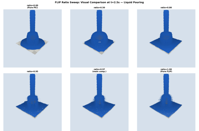
Fig. 10. FLIP ratio sweep visual comparison at t = 2.5s for the liquid-pouring scene. The same pattern holds: pure FLIP is noisy, pure PIC is overly damped, and ratios near 0.97 provide the most plausible visual behavior.
