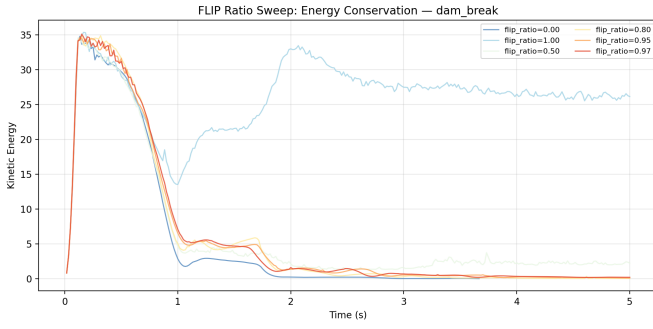
Fig. 6. Dam-break kinetic energy across FLIP blend ratios. Pure FLIP (ratio = 1.00) shows an explosive energy spike, while pure PIC (ratio = 0.00) dissipates energy almost immediately. The ratio = 0.97 used in the main comparison sits in a narrow effective window.
