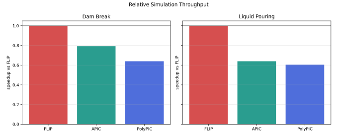
Fig. 14. Relative speedup normalized against FLIP within each scene. Values below 1 indicate slower runtime than the FLIP baseline.
