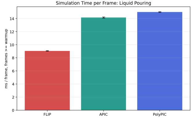
Fig. 13. Liquid-pouring simulation-only frame time. The same method ordering appears under the lower-particle-count scene.
