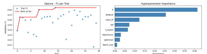
Fig. 2: Optuna Trials for Our Custom PyTorch Neural Network, ShotNet
