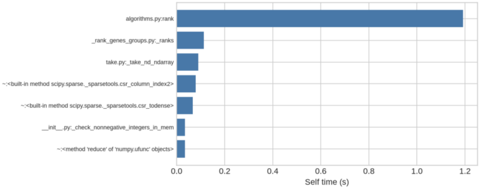
pbmc6k
