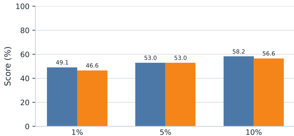
SQuAD v2 Exact Match
