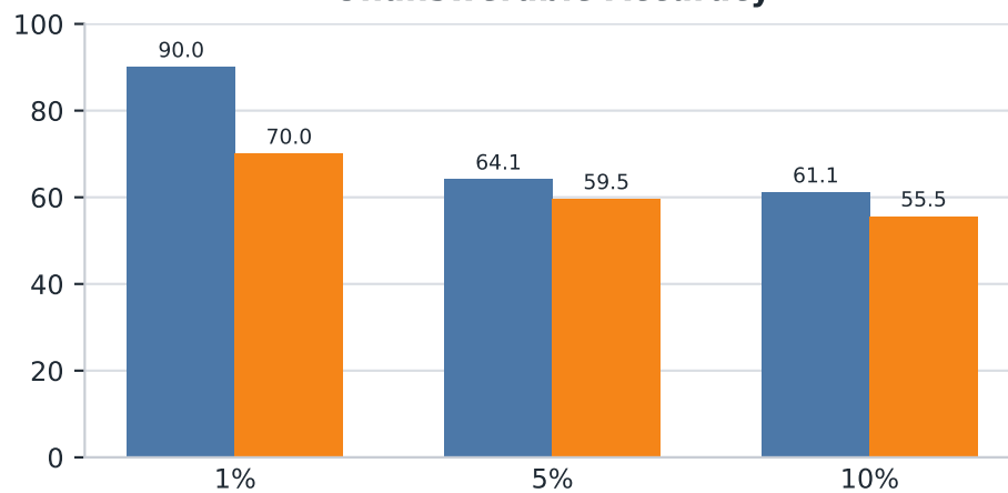
SQuAD v2 Unanswerable Accuracy
