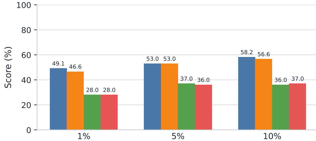
SQuAD v2 Exact Match
