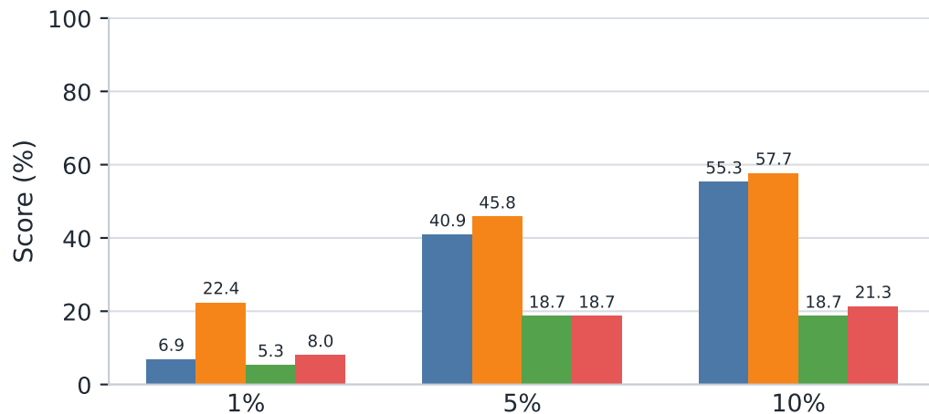
SQuAD v2 Answerable Exact Match
