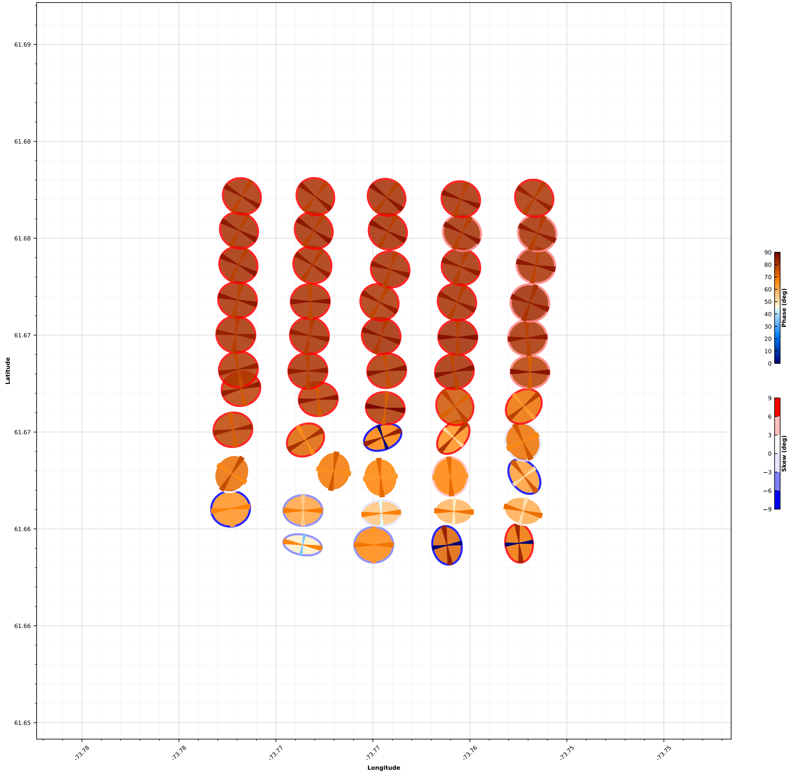
Phase Tensor Map for 0.042664 (s)
