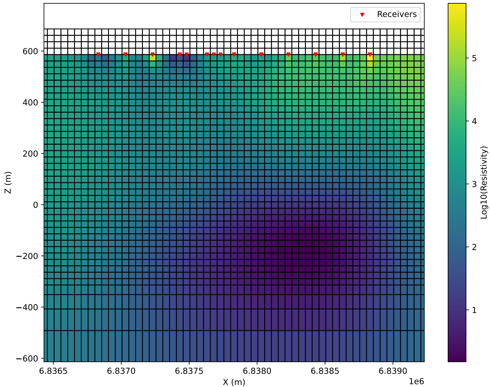
Model Slice — X = 565395.5 m
