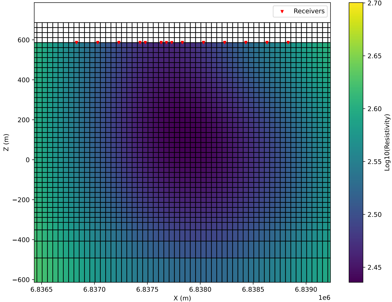
Model Slice — X = 563246.7 m
