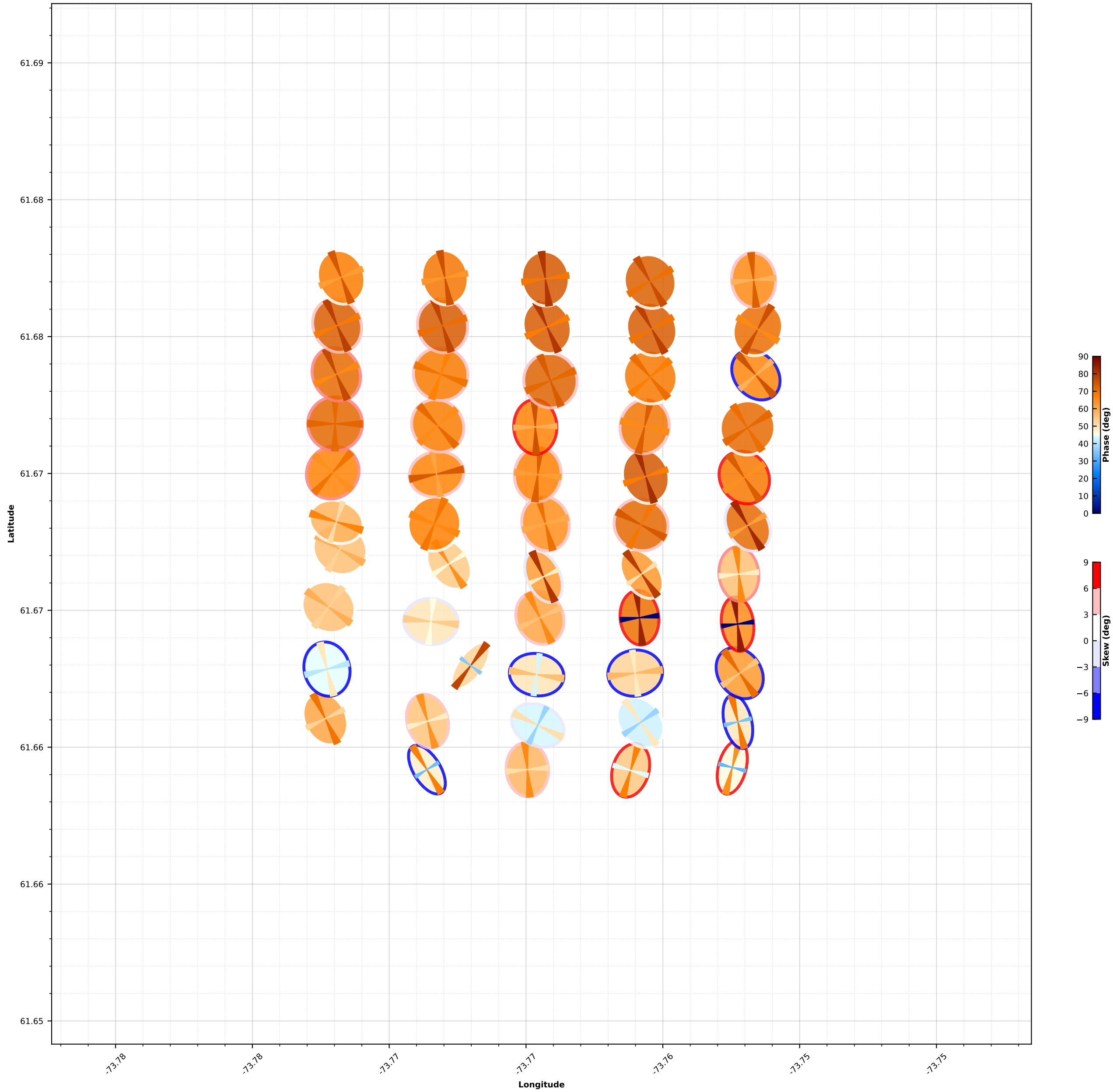
Phase Tensor Map for 0.0010158 (s)
