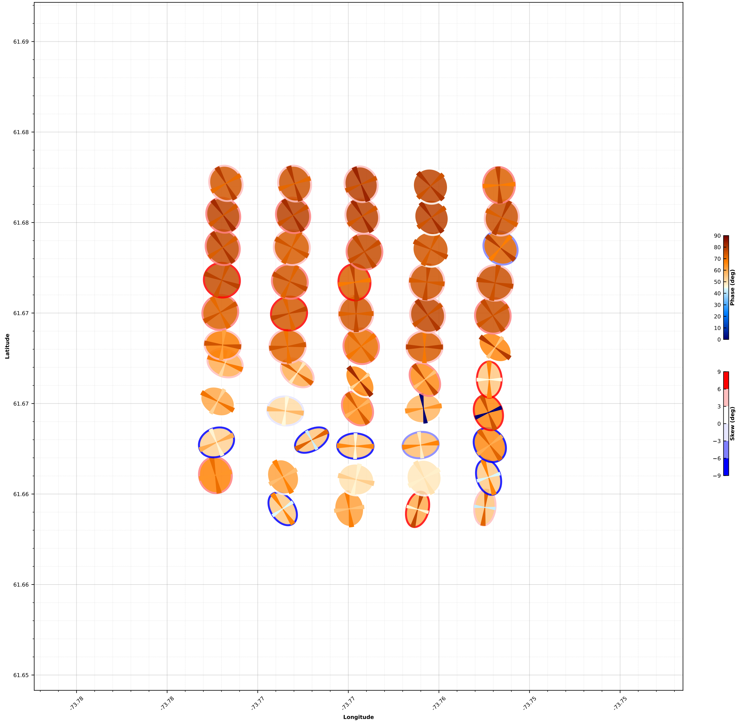
Phase Tensor Map for 0.0023061 (s)
