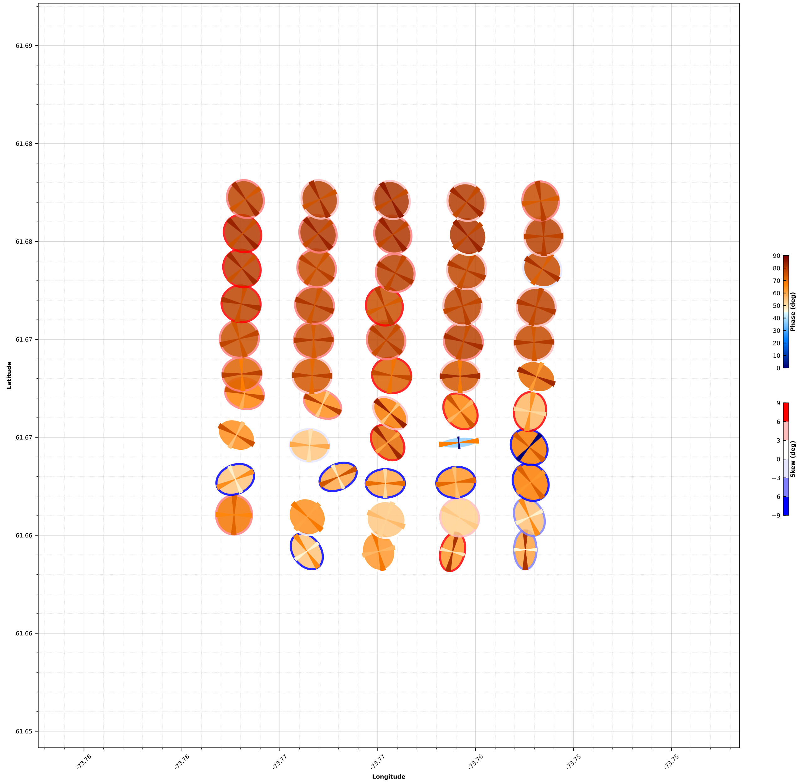
Phase Tensor Map for 0.0042662 (s)
