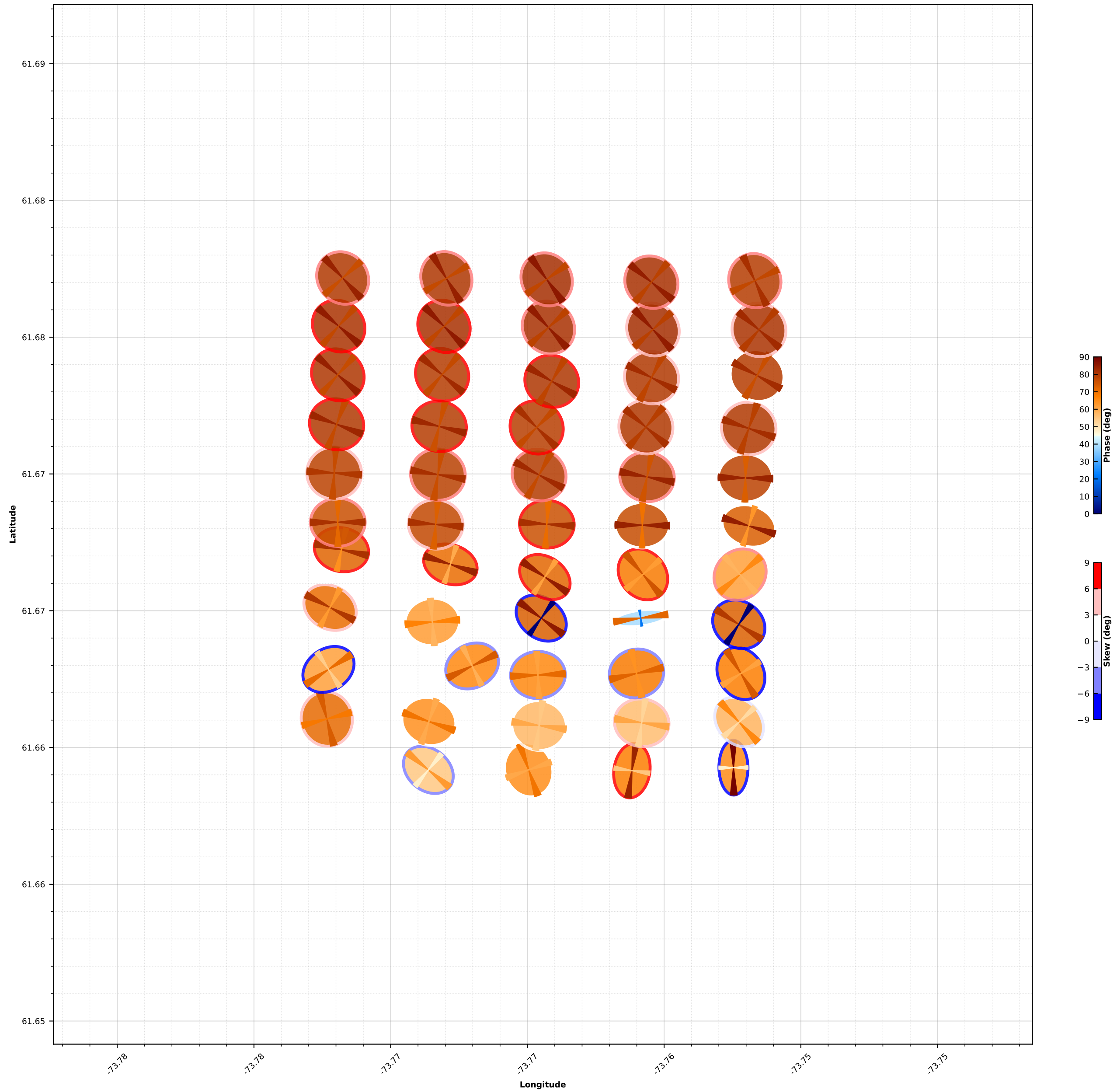
Phase Tensor Map for 0.010037 (s)
