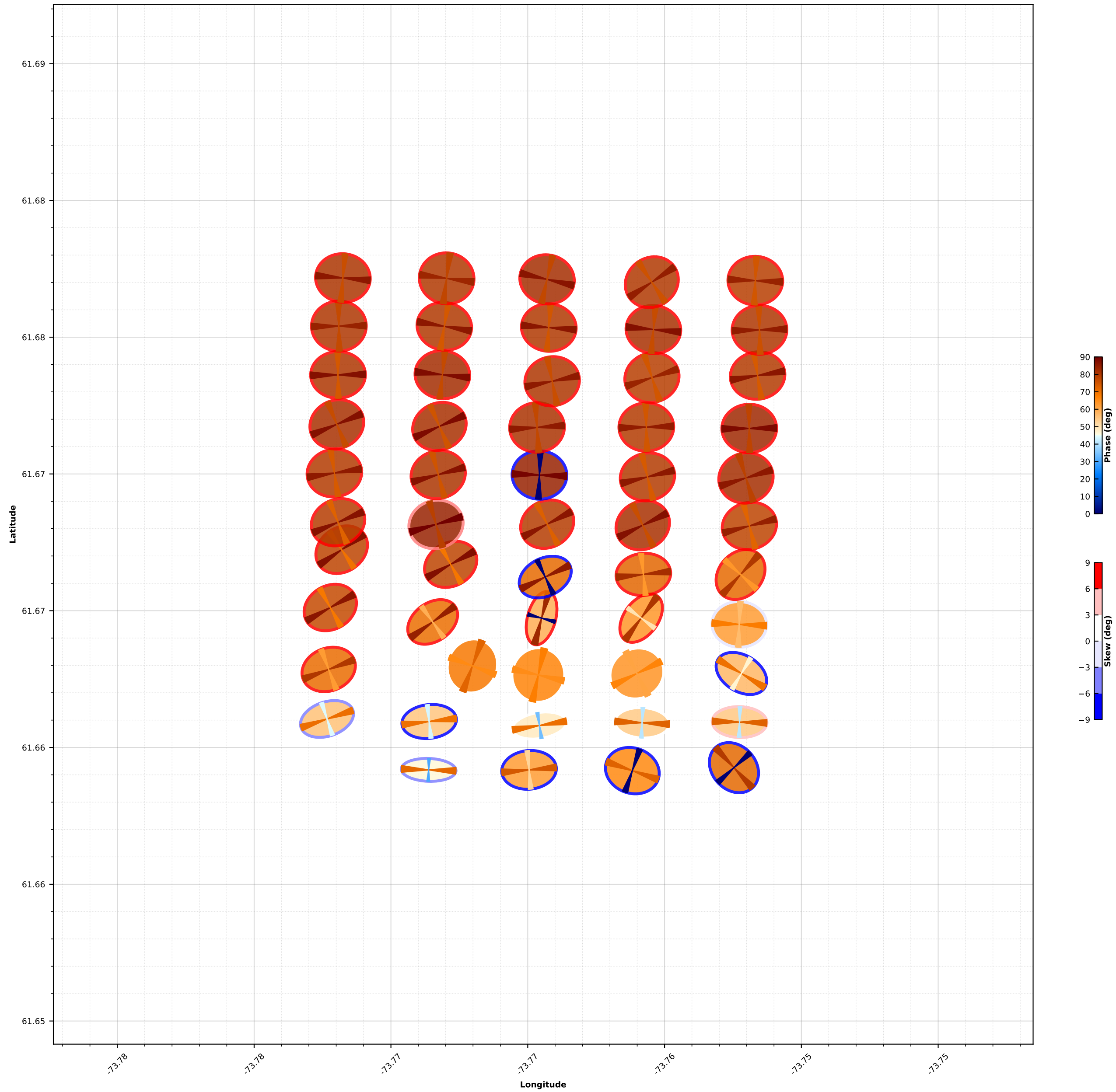
Phase Tensor Map for 0.12412 (s)
