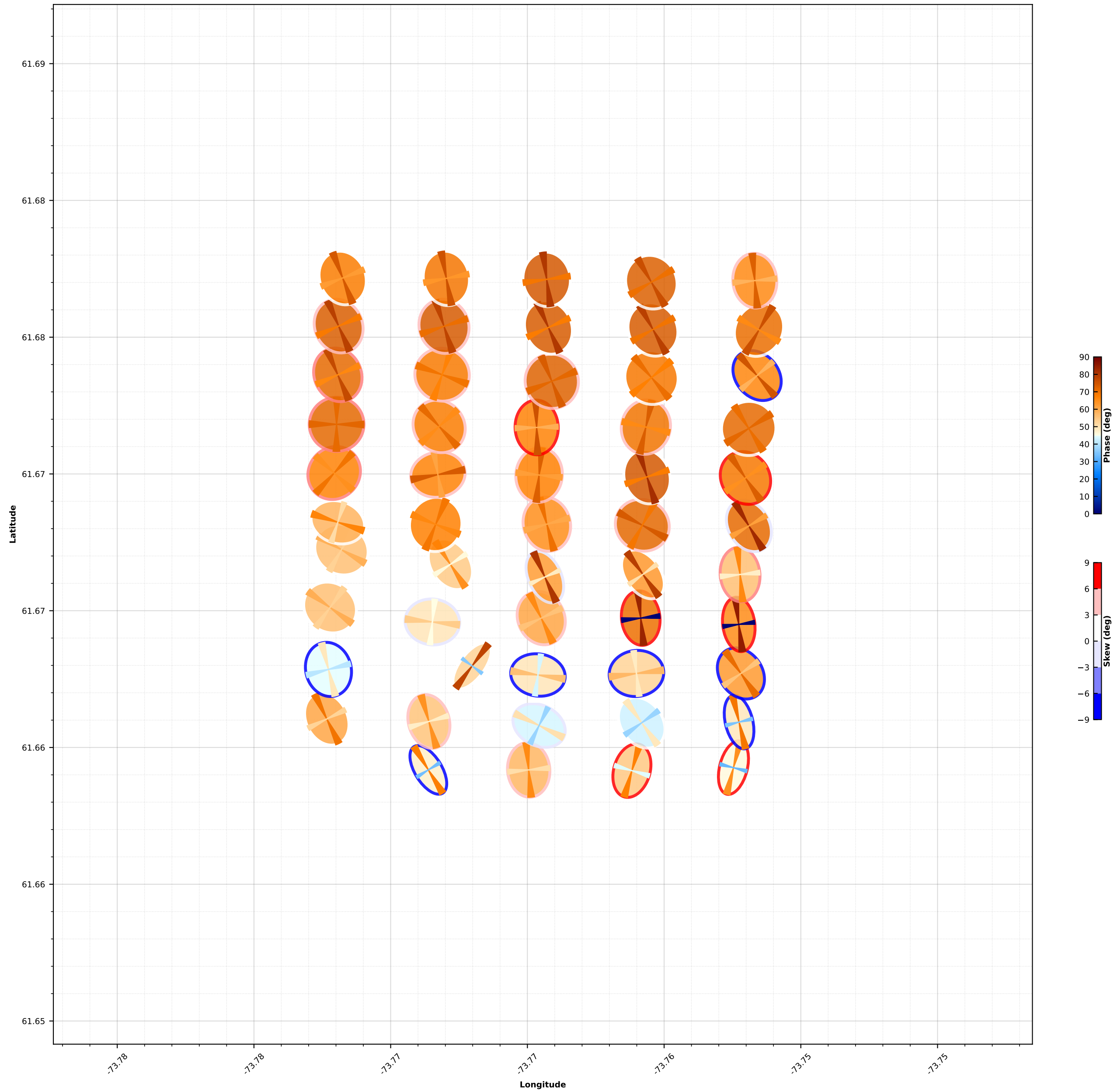
Phase Tensor Map for 0.0010158 (s)
