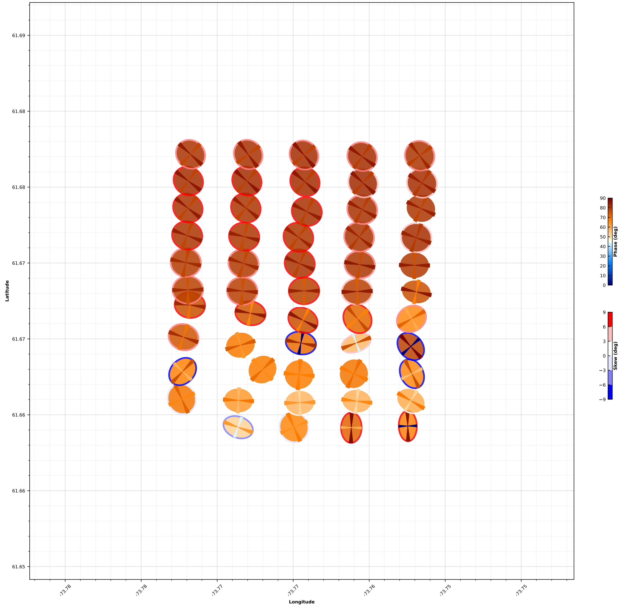
Phase Tensor Map for 0.018958 (s)
