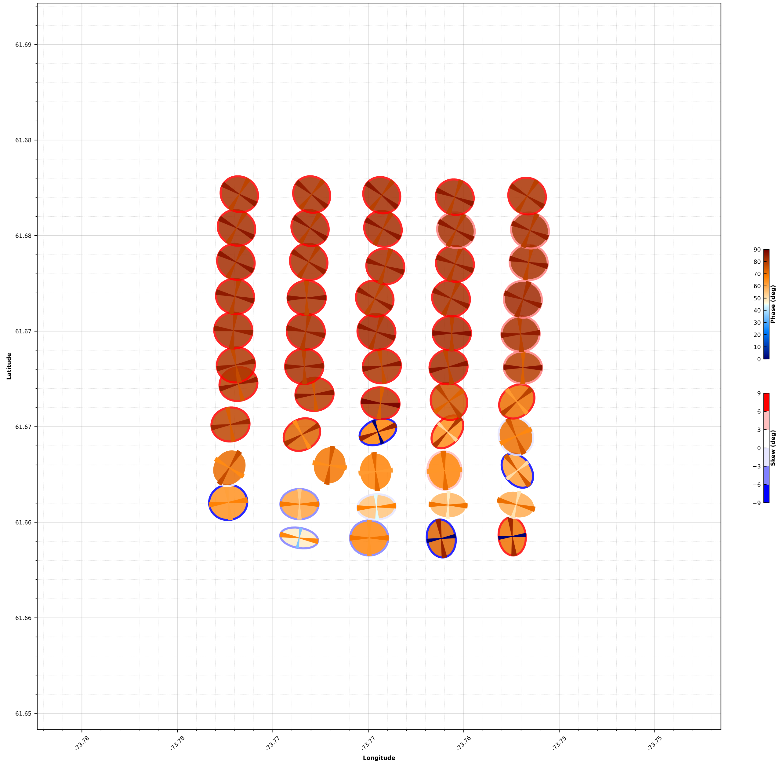
Phase Tensor Map for 0.042664 (s)
