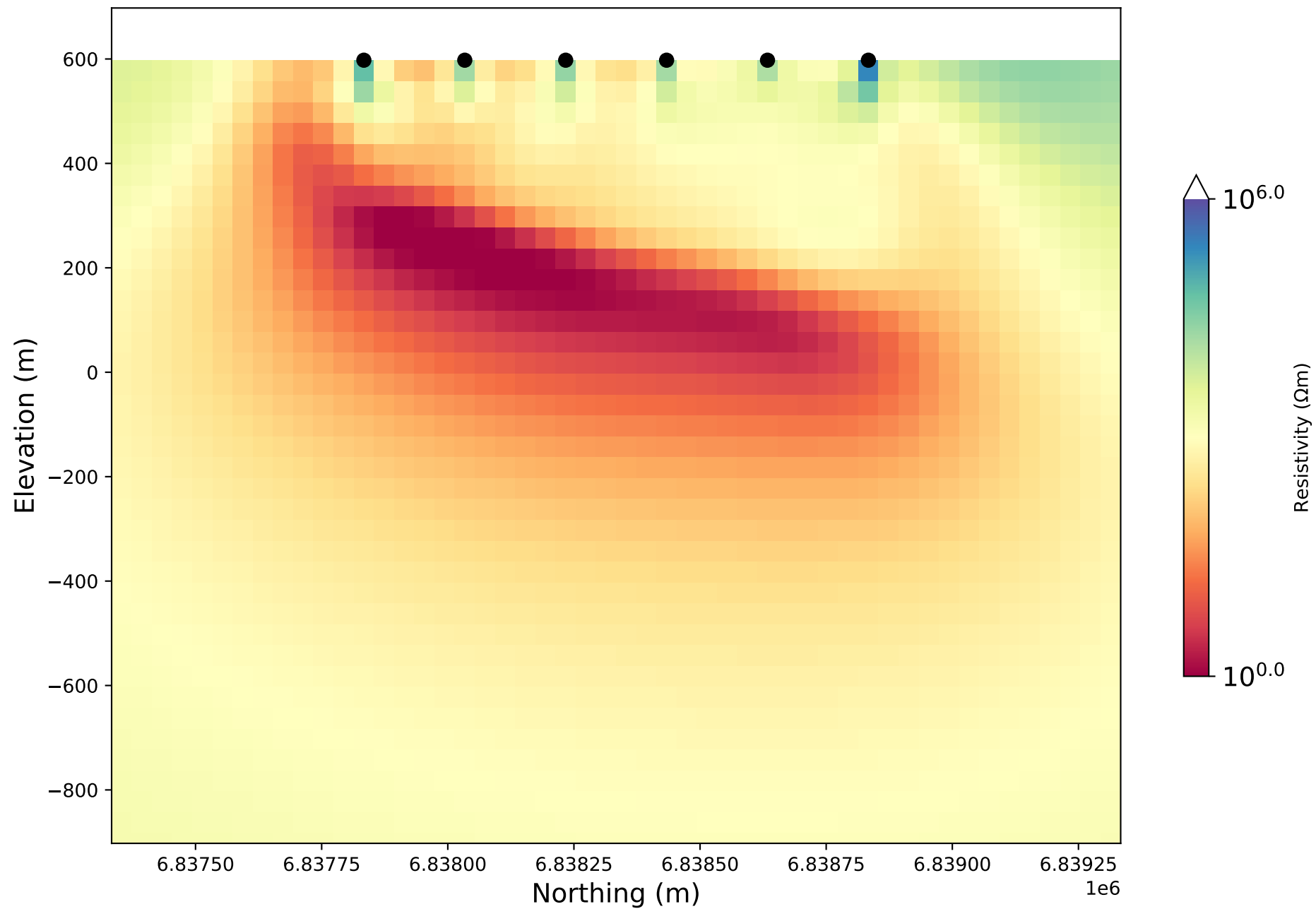
2D Inversion Results - P01cf
