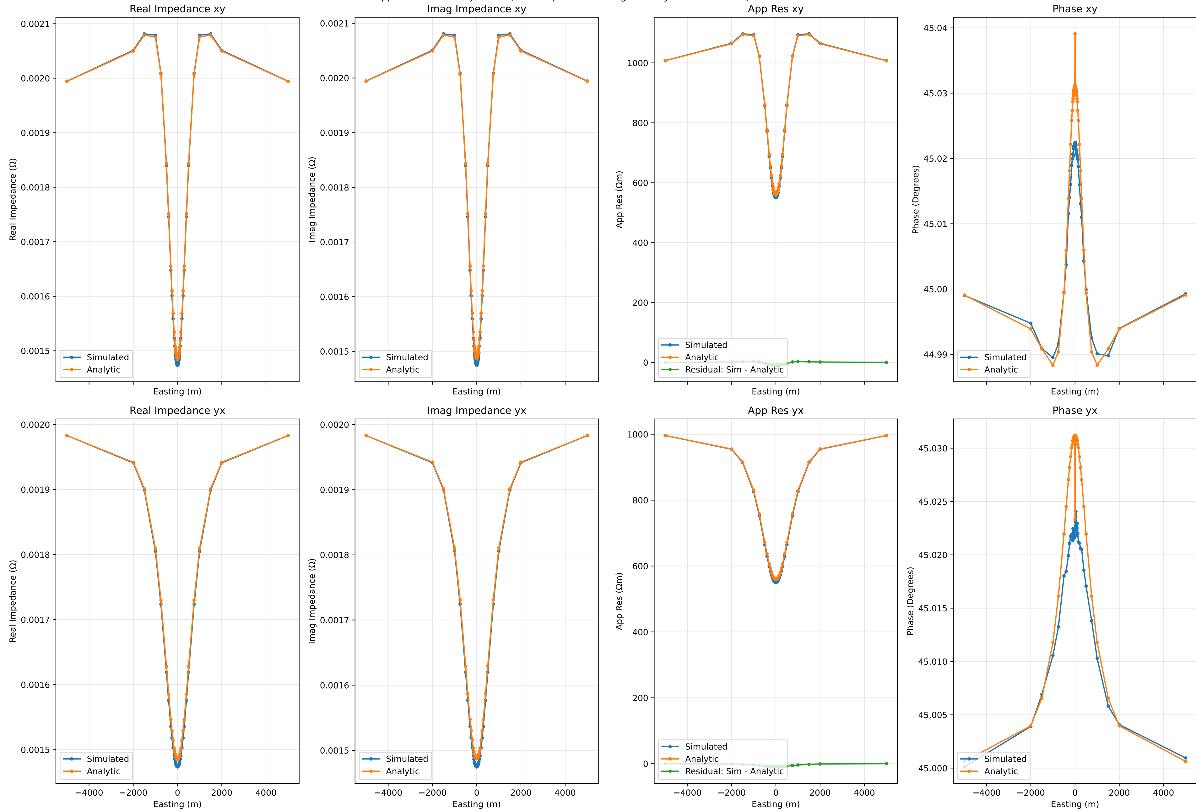
Apparent Resistivity, Phase, and Impedance along Cut at y=0 for 0.001Hz, Run Number 41
