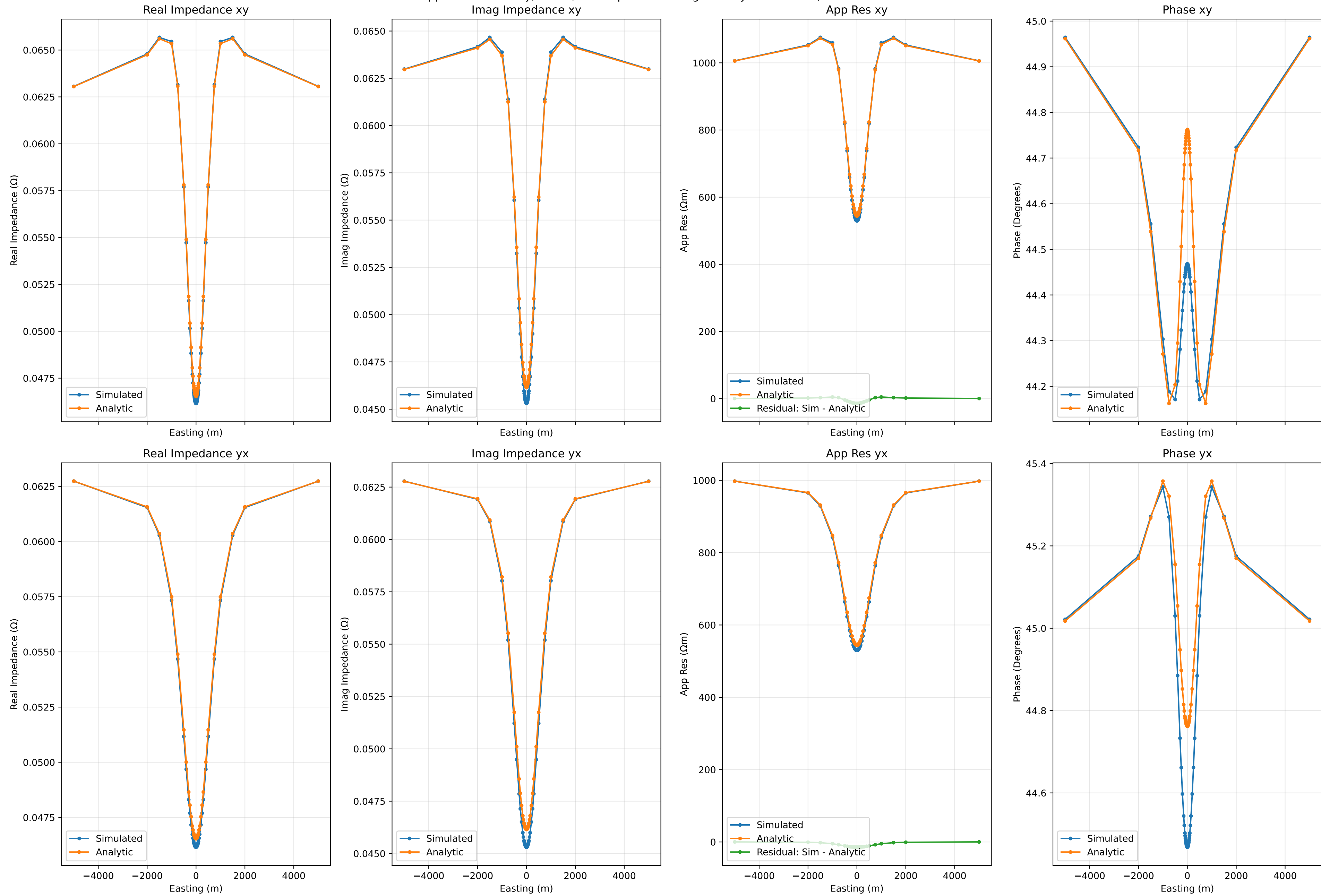
Apparent Resistivity, Phase, and Impedance along Cut at y=0 for 1.0Hz, Run Number 42
