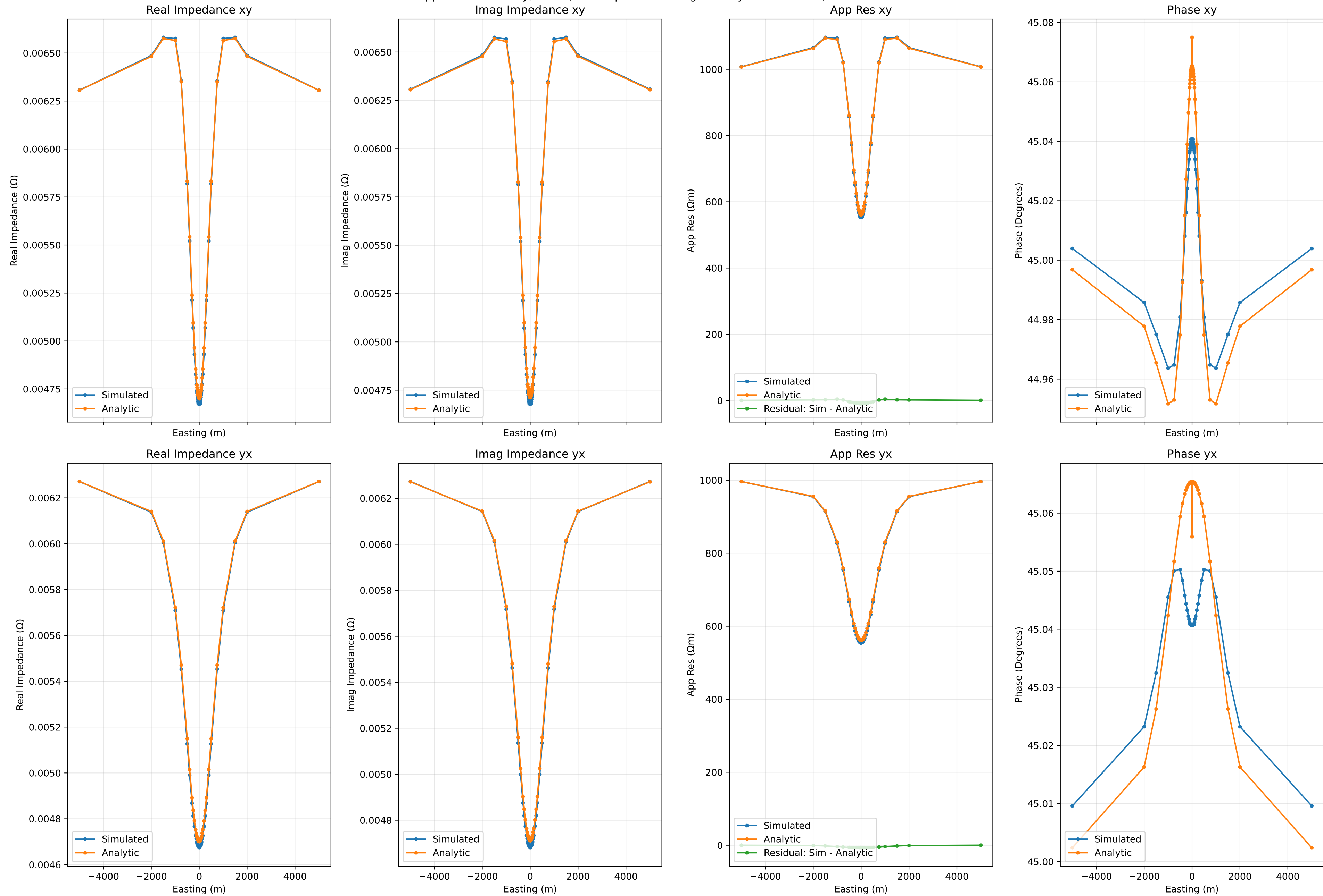
Apparent Resistivity, Phase, and Impedance along Cut at y=0 for 0.01Hz, Run Number 46
