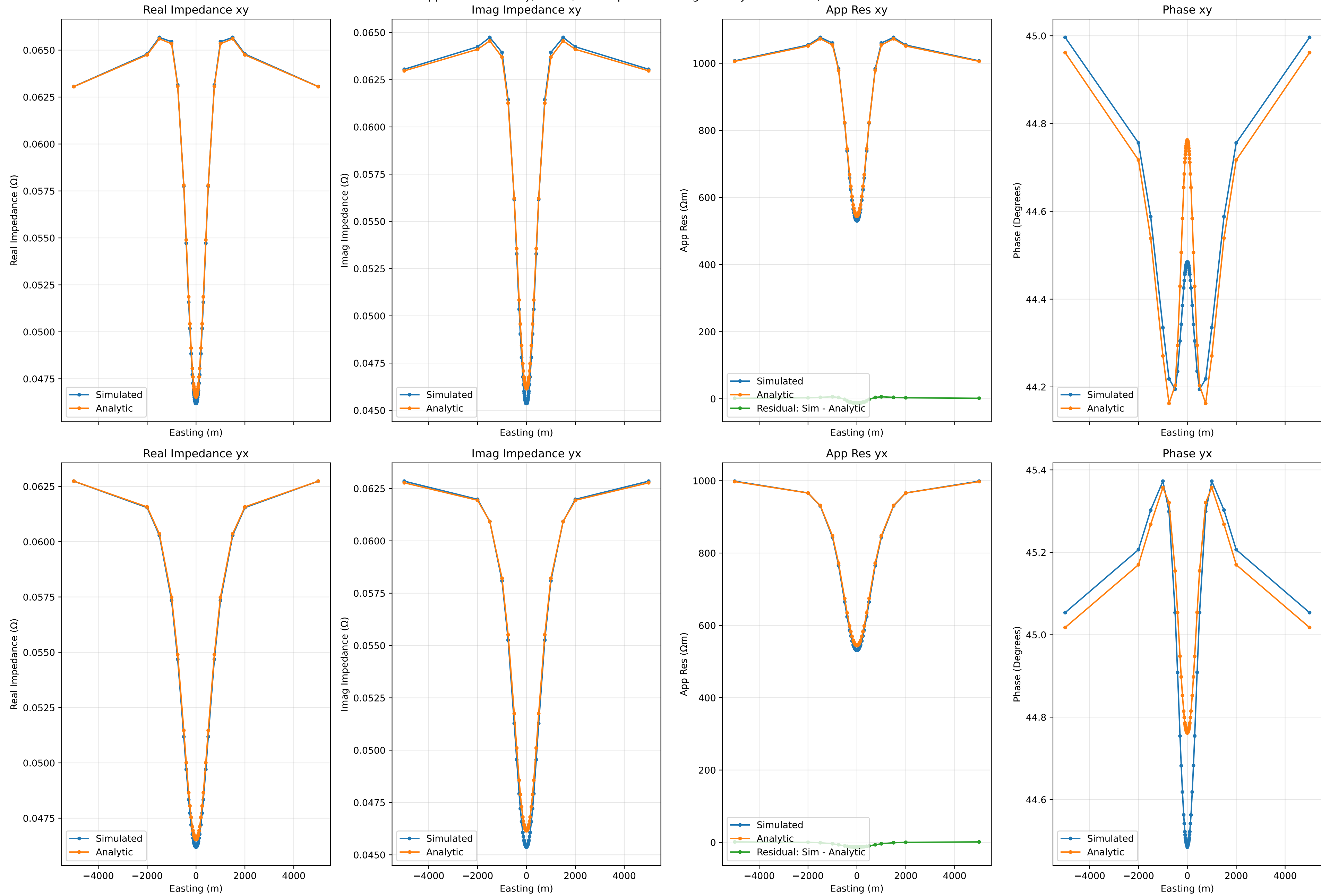
Apparent Resistivity, Phase, and Impedance along Cut at y=0 for 1.0Hz, Run Number 45
