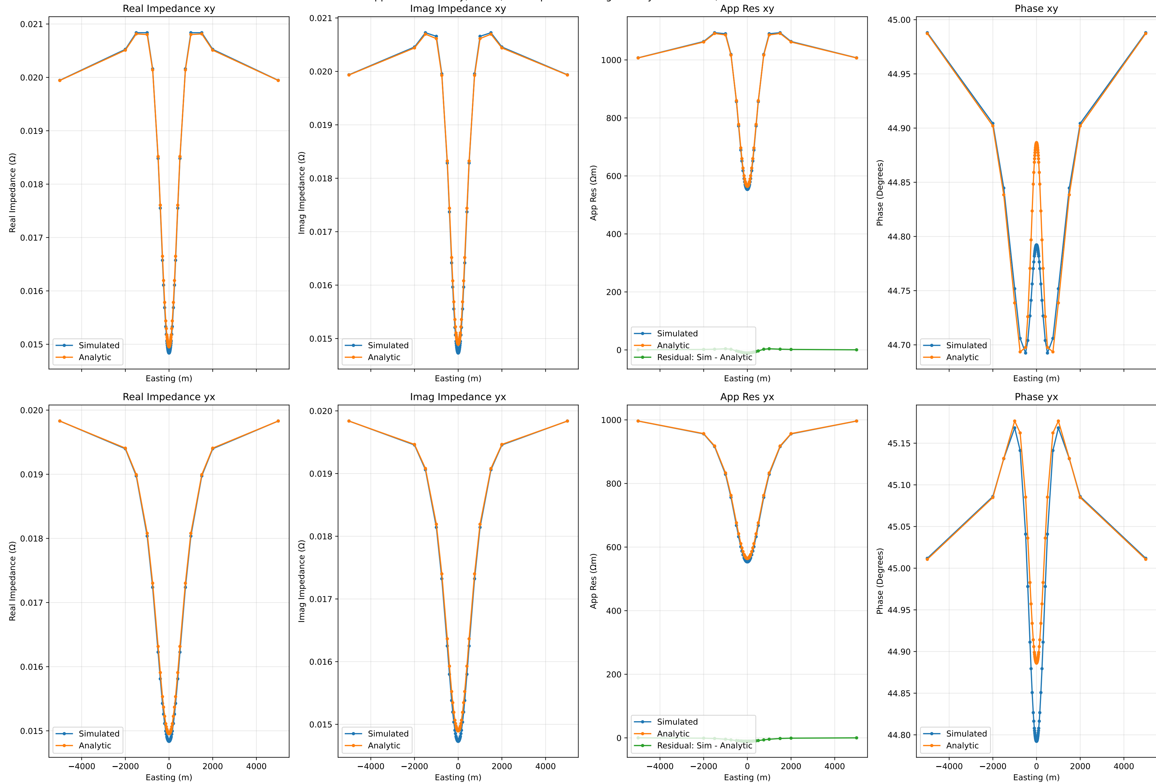
Apparent Resistivity, Phase, and Impedance along Cut at y=0 for 0.1Hz, Run Number 42
