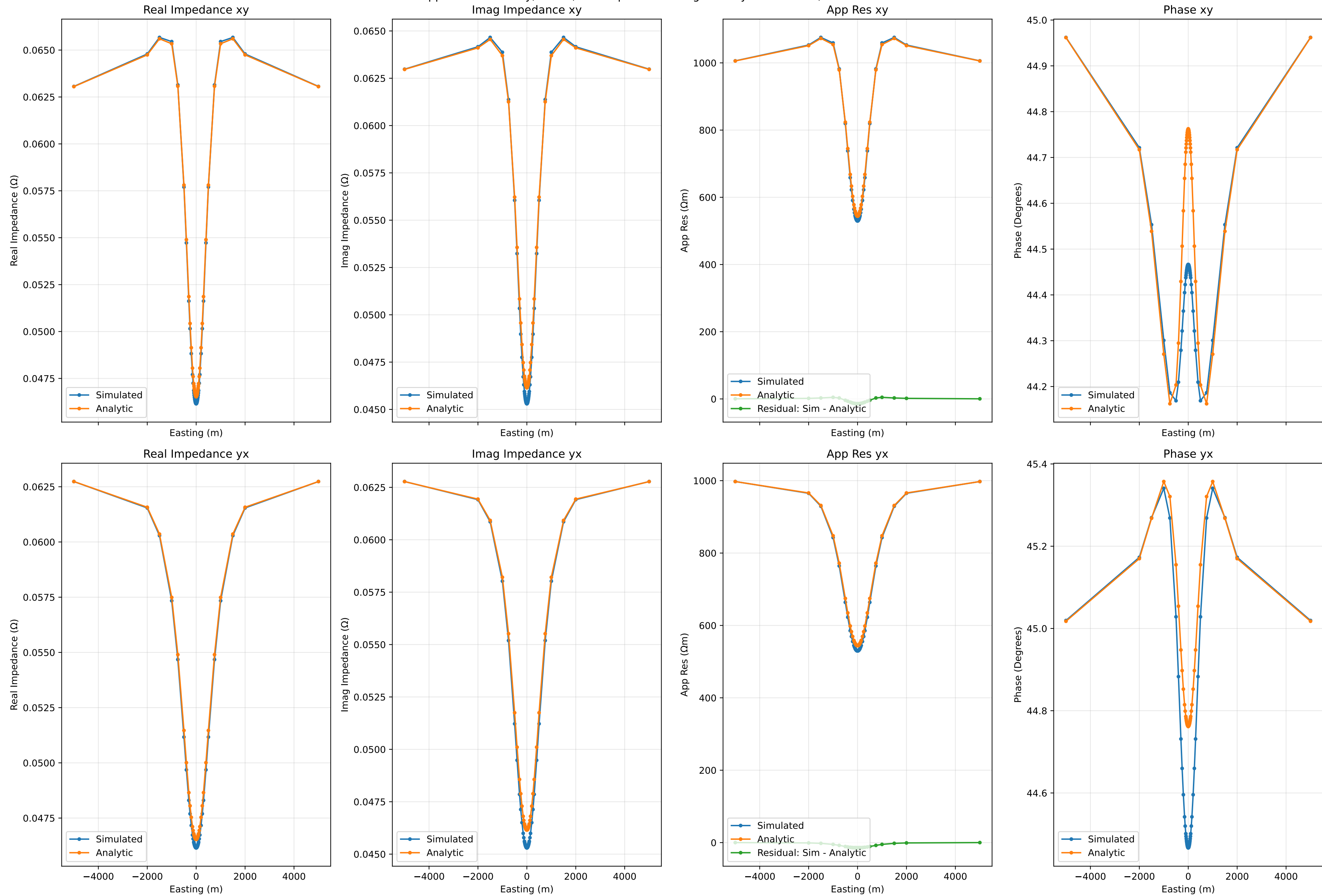
Apparent Resistivity, Phase, and Impedance along Cut at y=0 for 1.0Hz, Run Number 41
