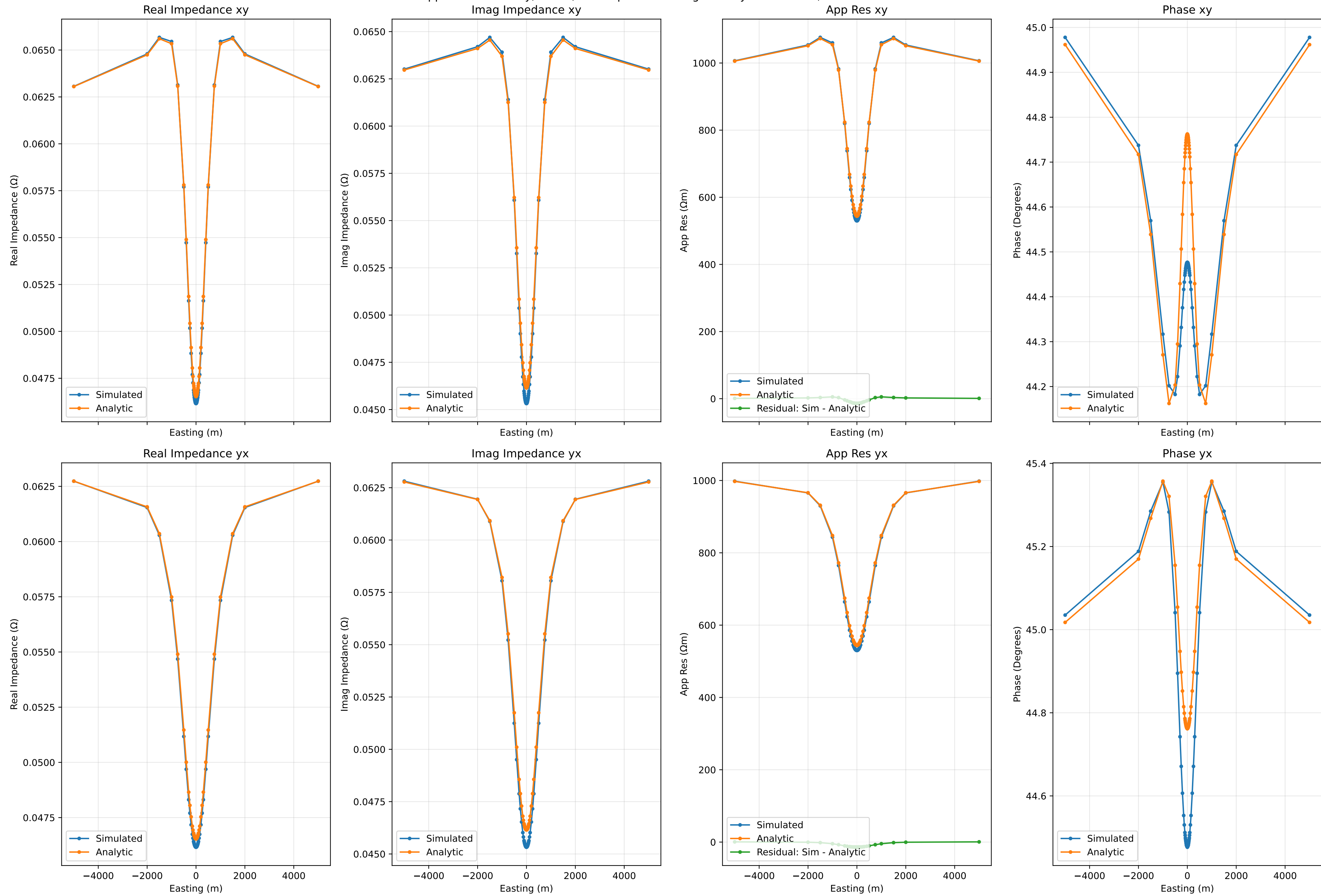
Apparent Resistivity, Phase, and Impedance along Cut at y=0 for 1.0Hz, Run Number 44
