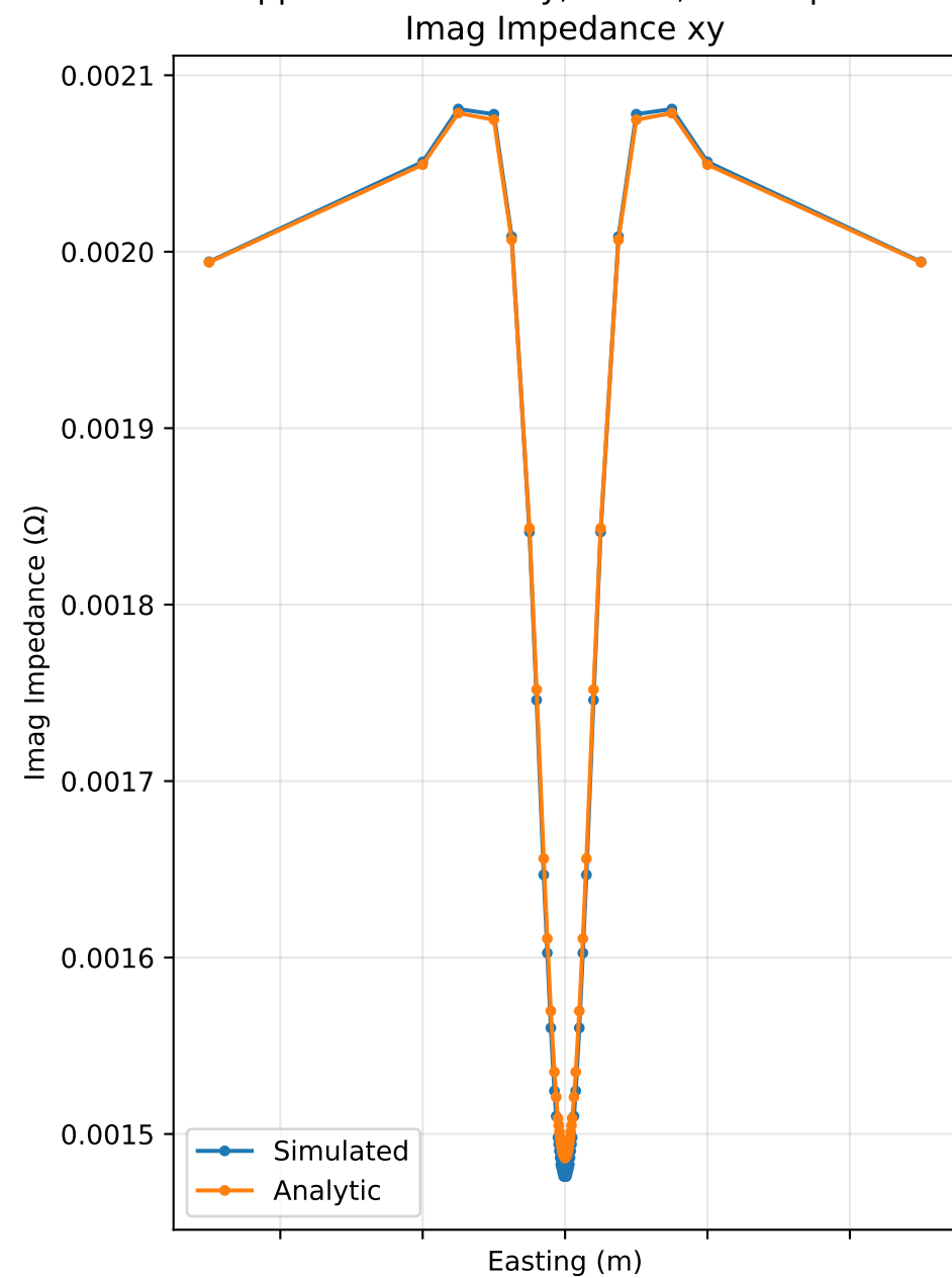
Apparent Resistivity, Phase, and Impedance along Cut at y=0 for 0.001Hz, Run Number 45
