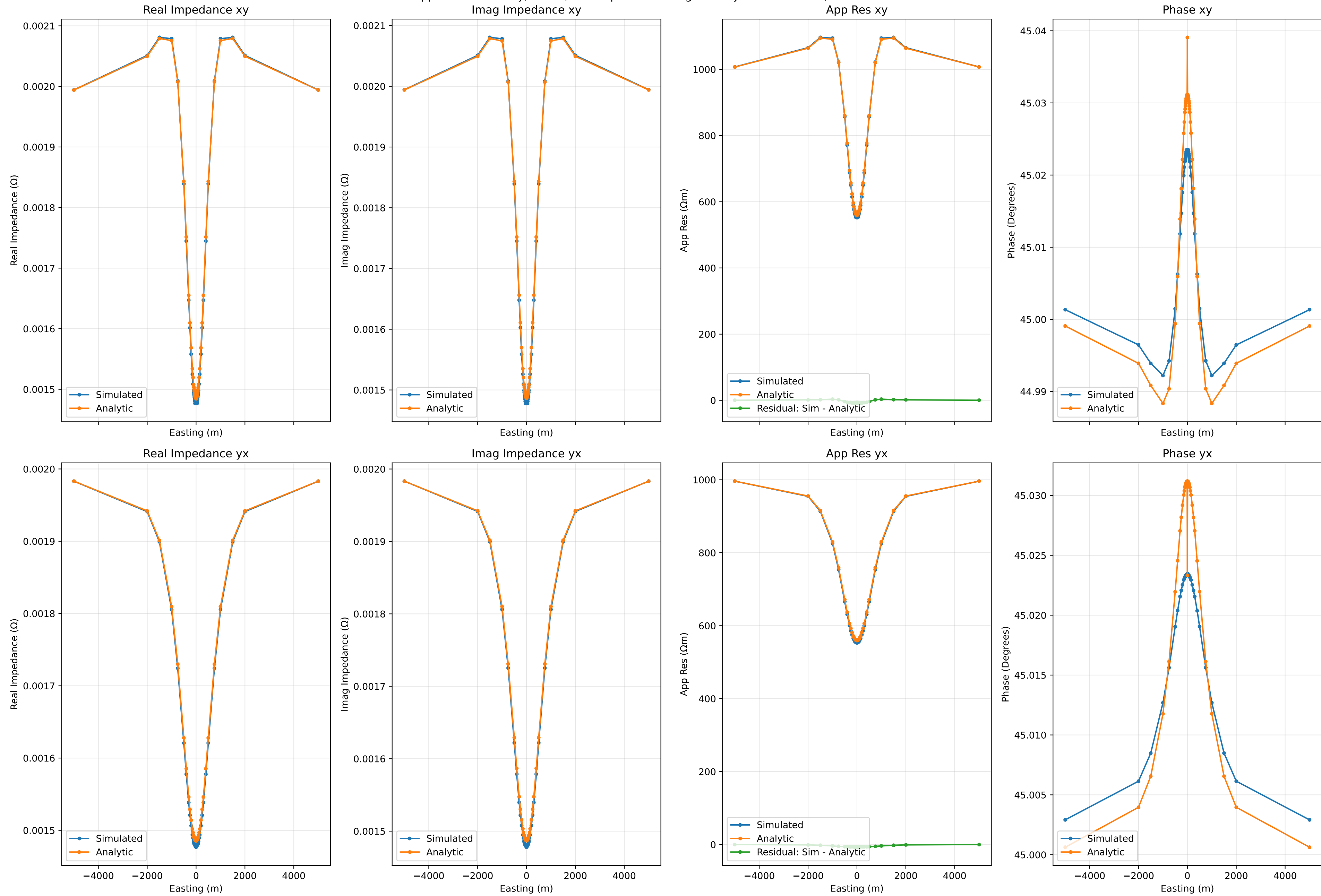
Apparent Resistivity, Phase, and Impedance along Cut at y=0 for 0.001Hz, Run Number 46
