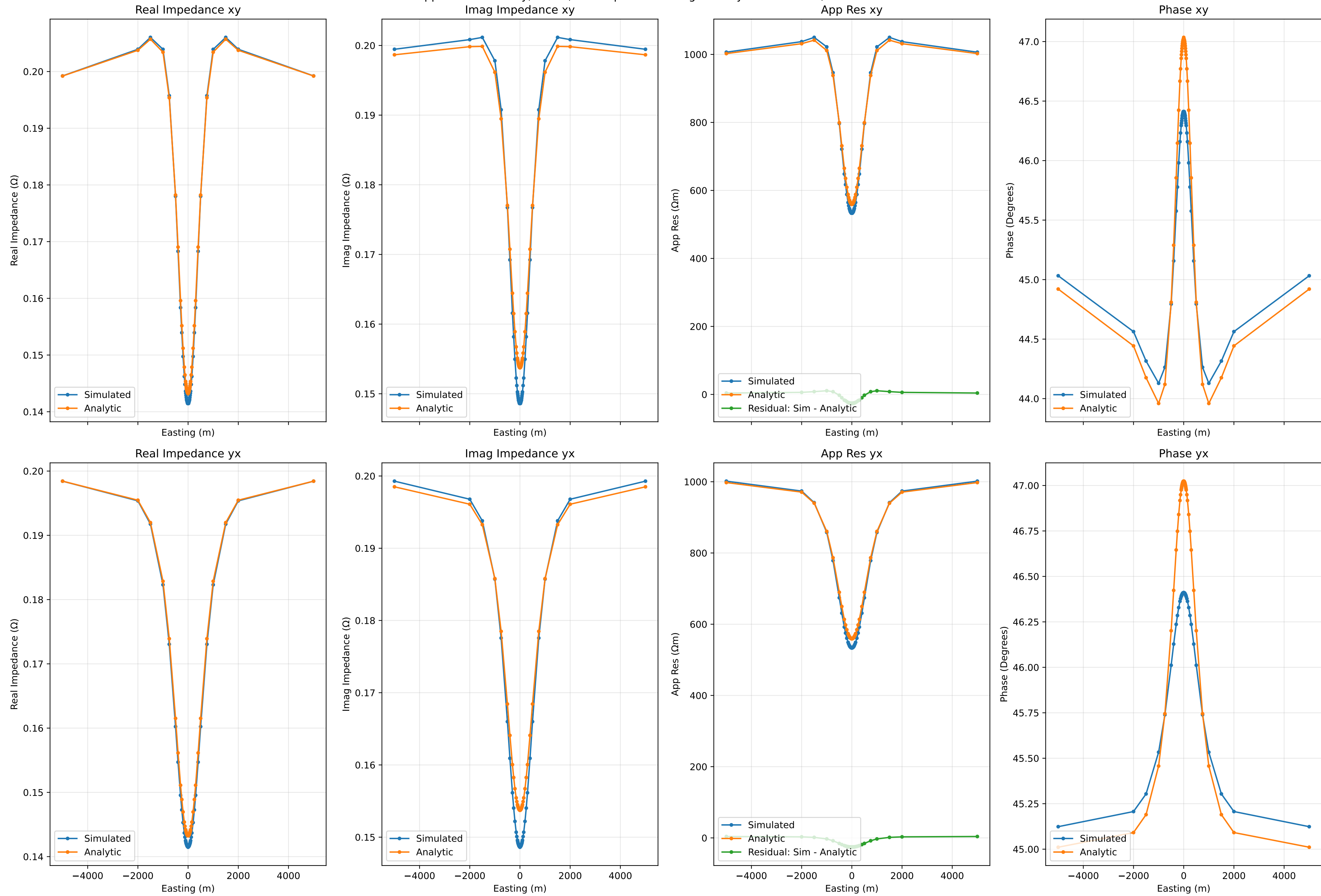
Apparent Resistivity, Phase, and Impedance along Cut at y=0 for 10.0Hz, Run Number 45
