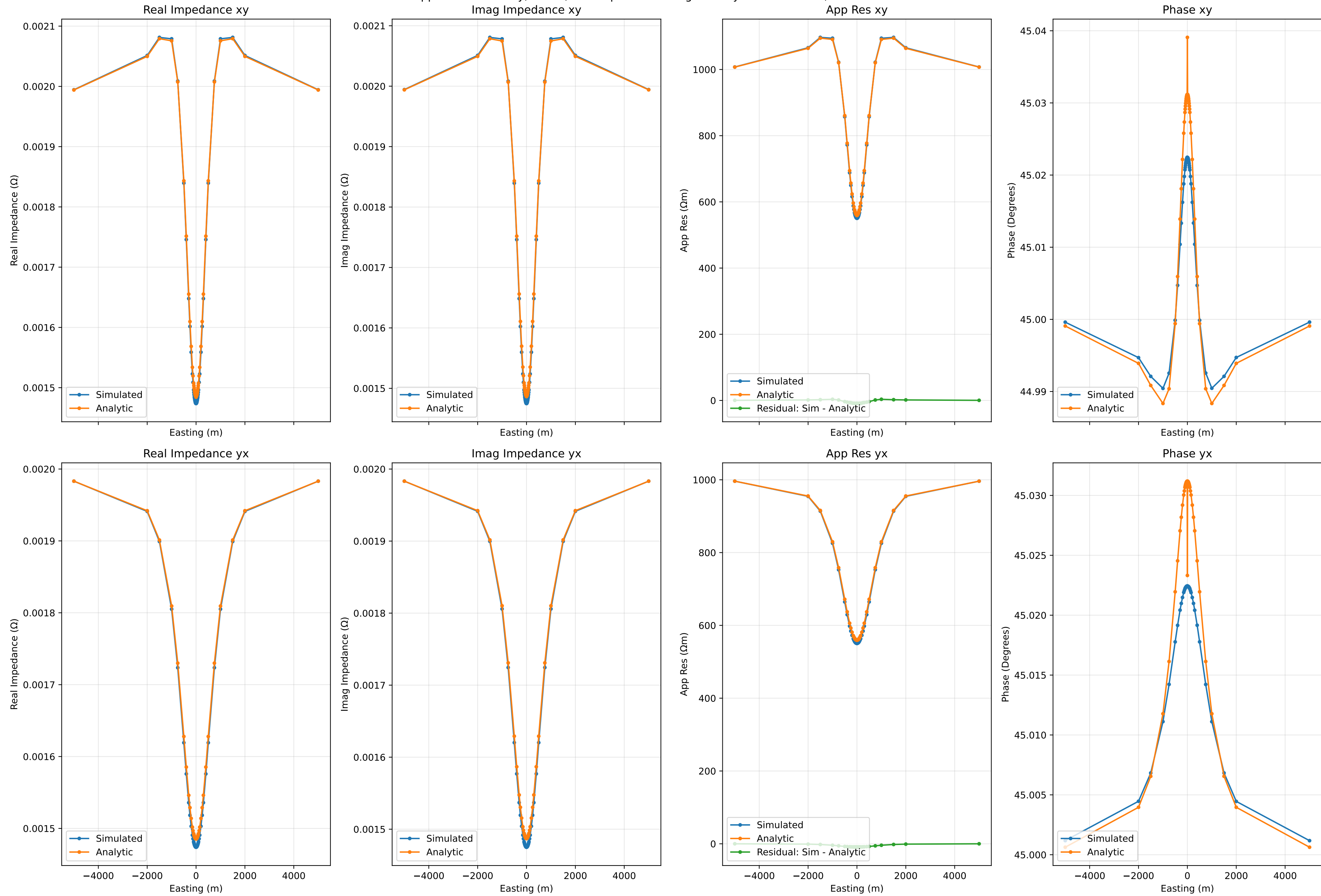
Apparent Resistivity, Phase, and Impedance along Cut at y=0 for 0.001Hz, Run Number 44
