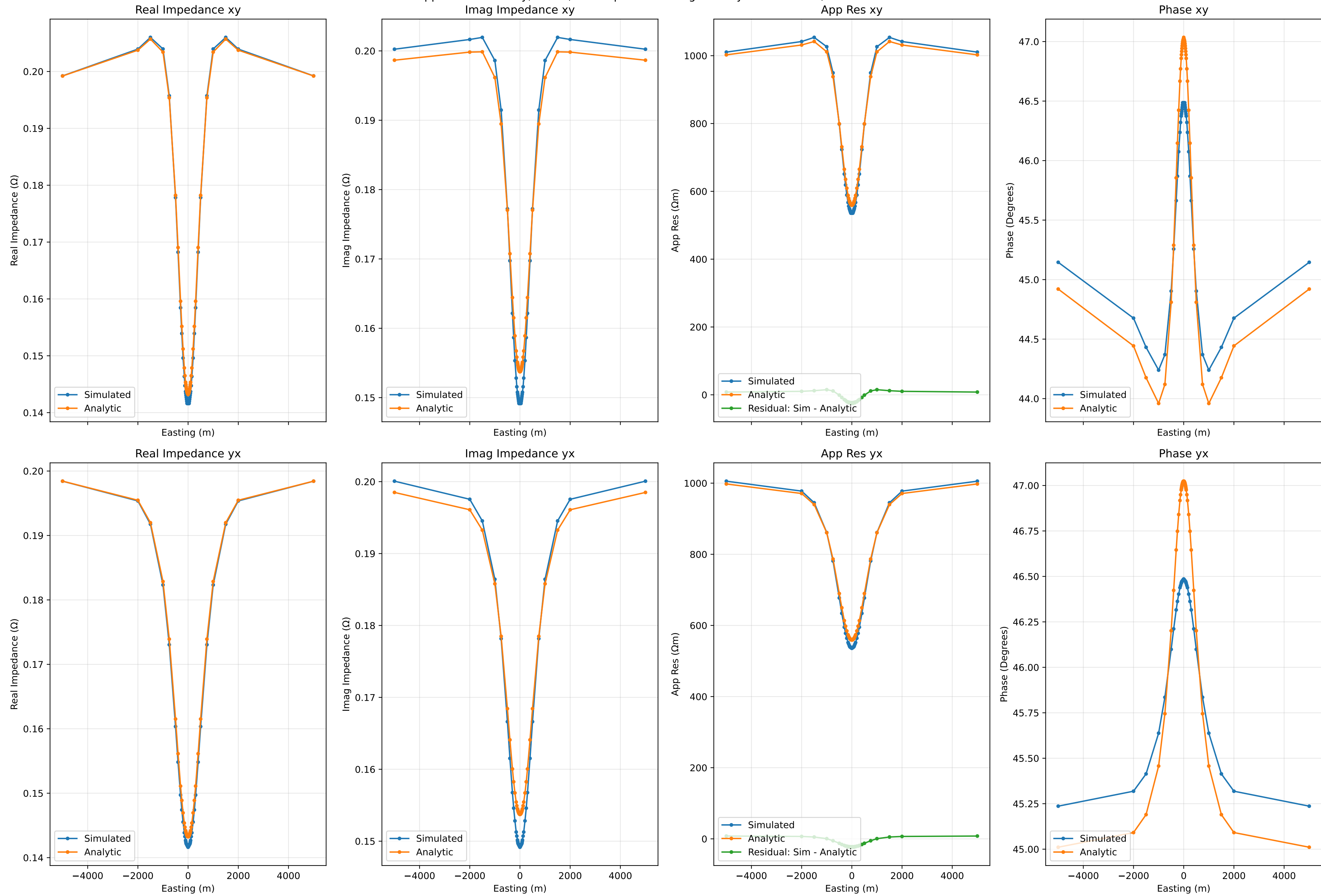
Apparent Resistivity, Phase, and Impedance along Cut at y=0 for 10.0Hz, Run Number 46
