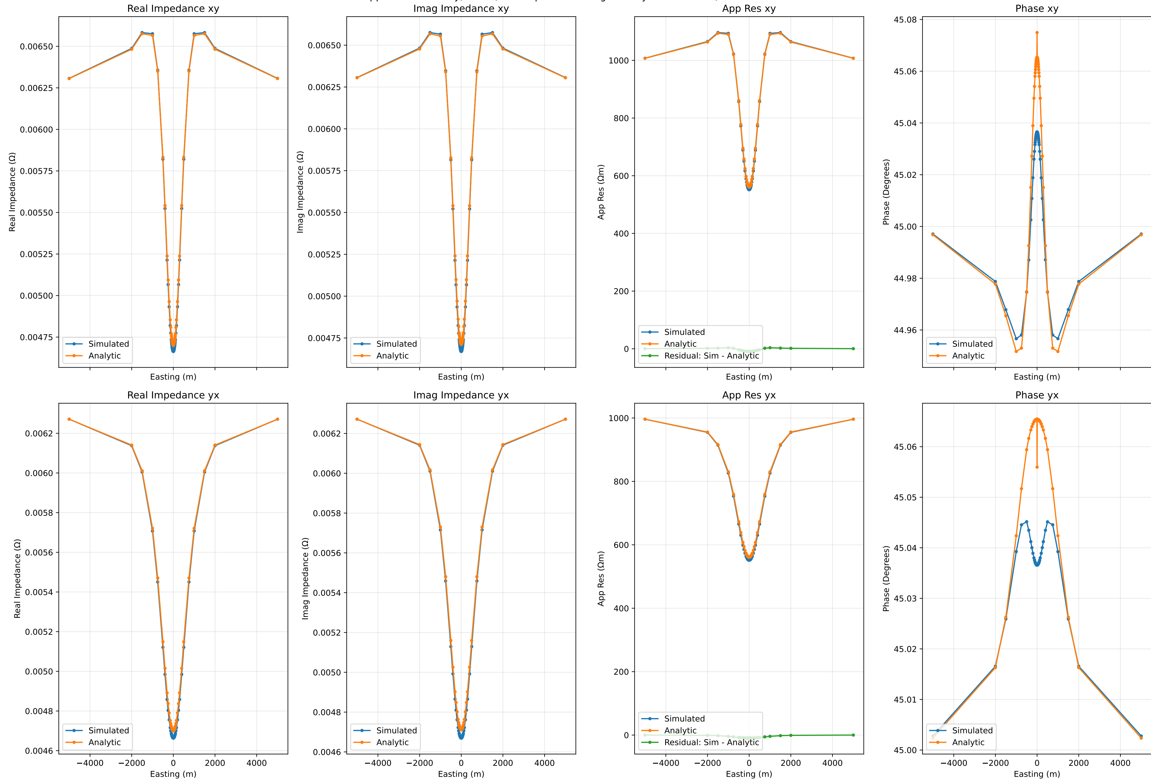
Apparent Resistivity, Phase, and Impedance along Cut at y=0 for 0.01Hz, Run Number 42
