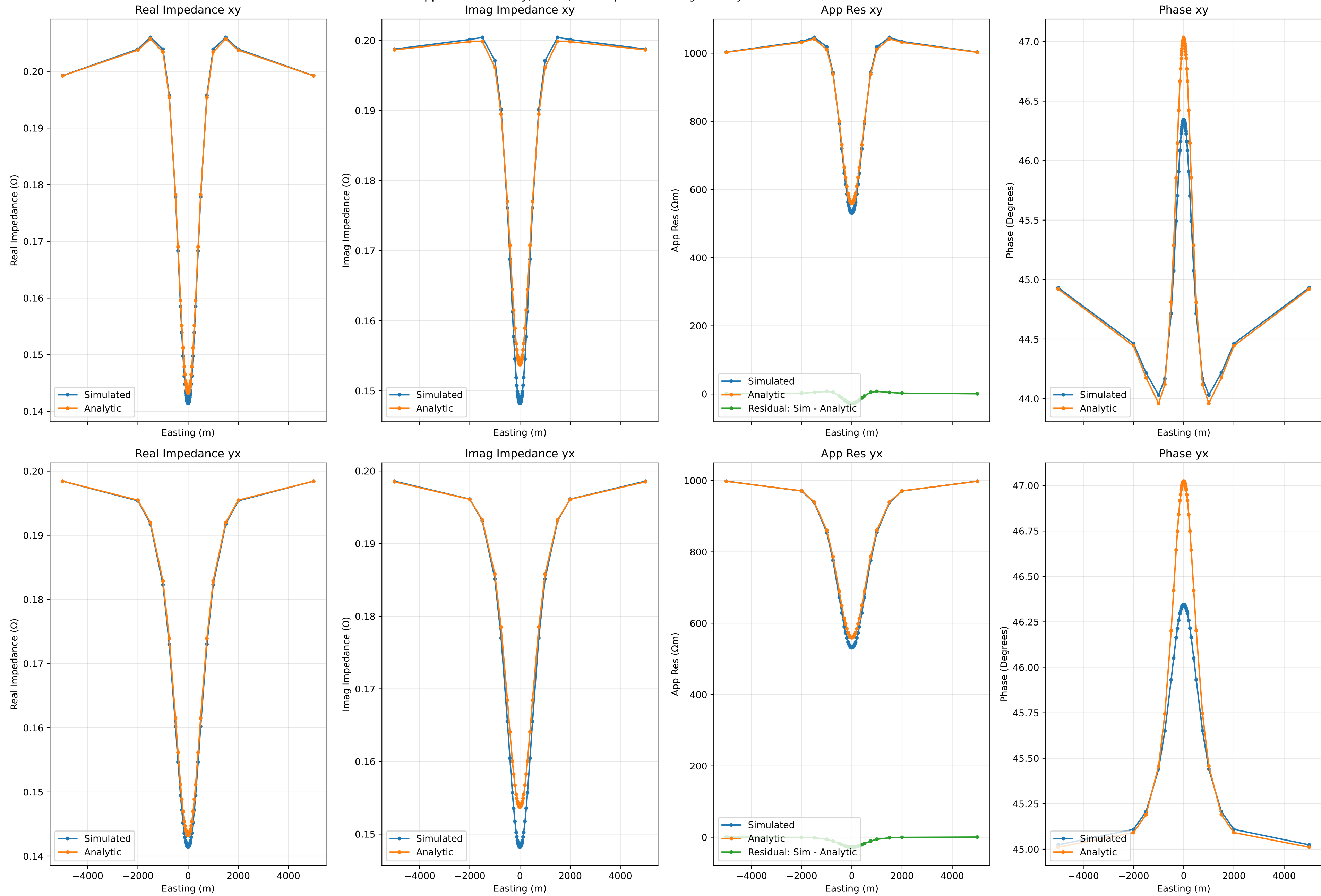
Apparent Resistivity, Phase, and Impedance along Cut at y=0 for 10.0Hz, Run Number 42
