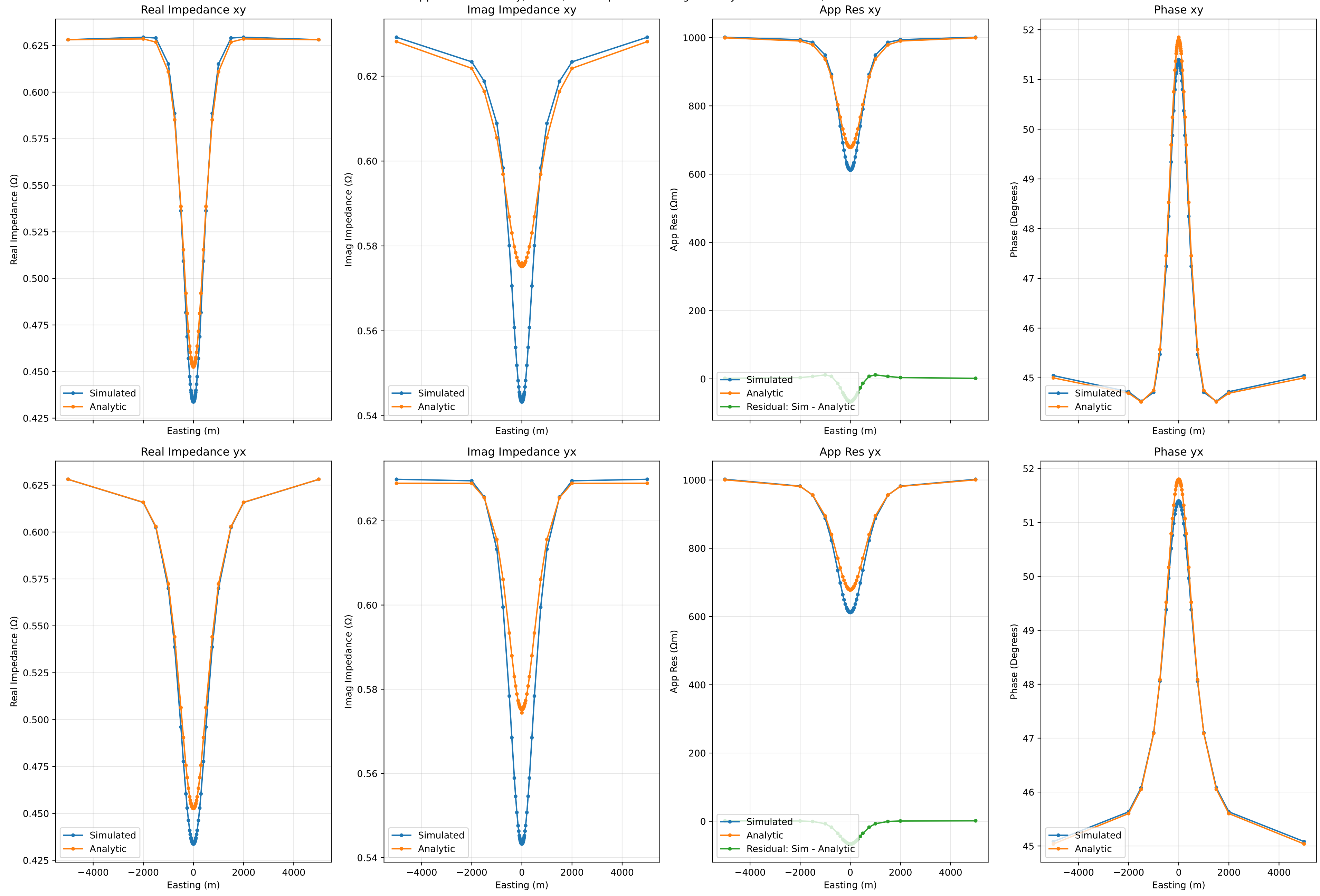
Apparent Resistivity, Phase, and Impedance along Cut at y=0 for 100.0Hz, Run Number 42
