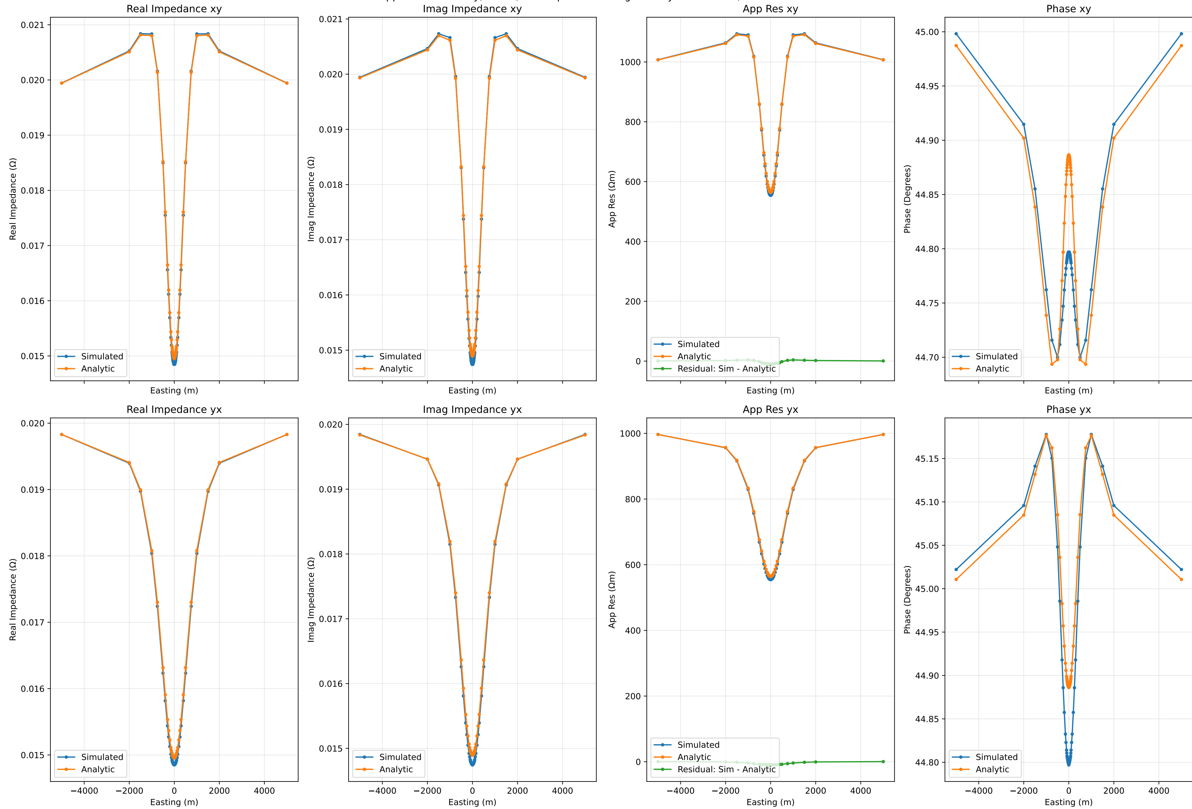
Apparent Resistivity, Phase, and Impedance along Cut at y=0 for 0.1Hz, Run Number 45
