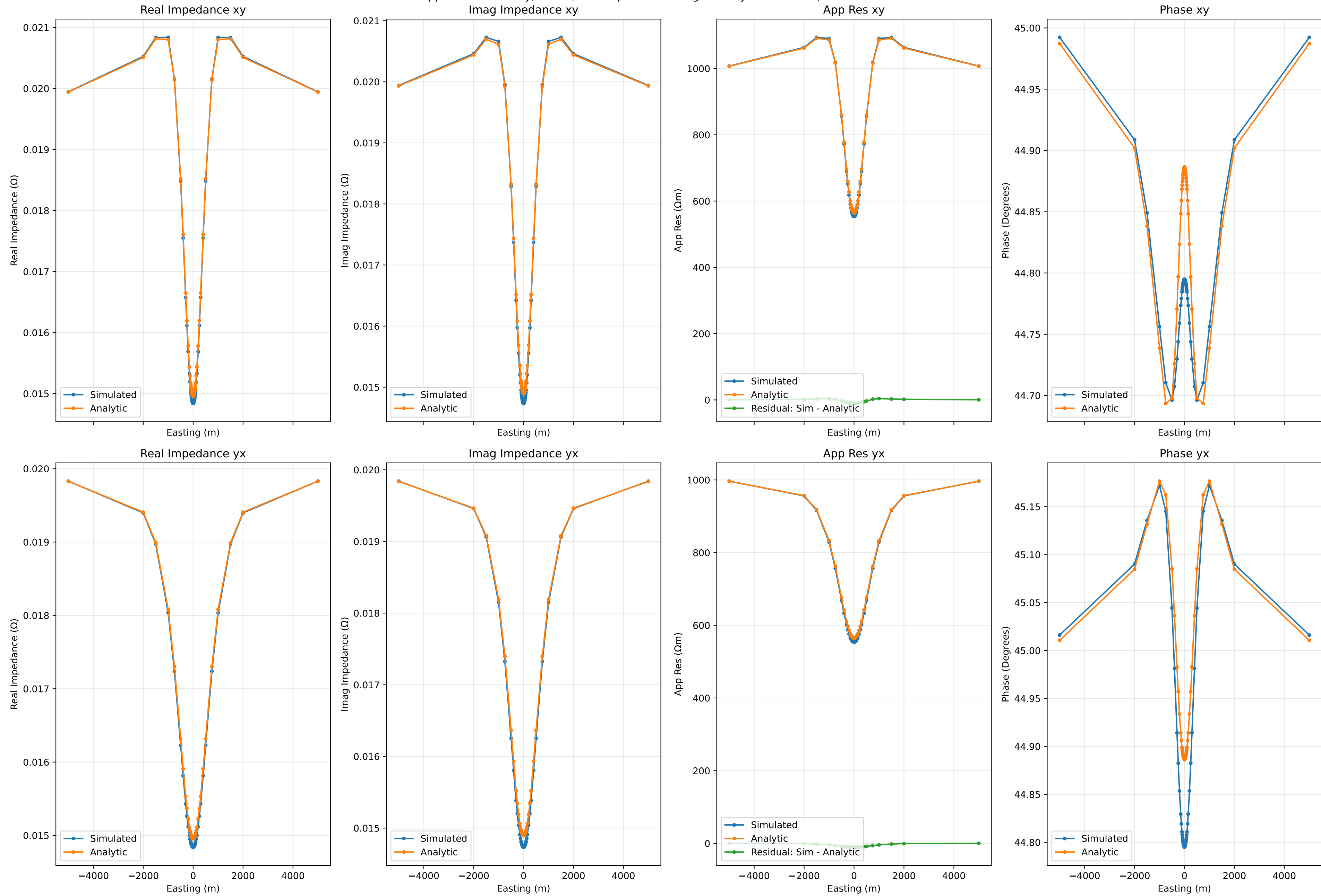
Apparent Resistivity, Phase, and Impedance along Cut at y=0 for 0.1Hz, Run Number 44
