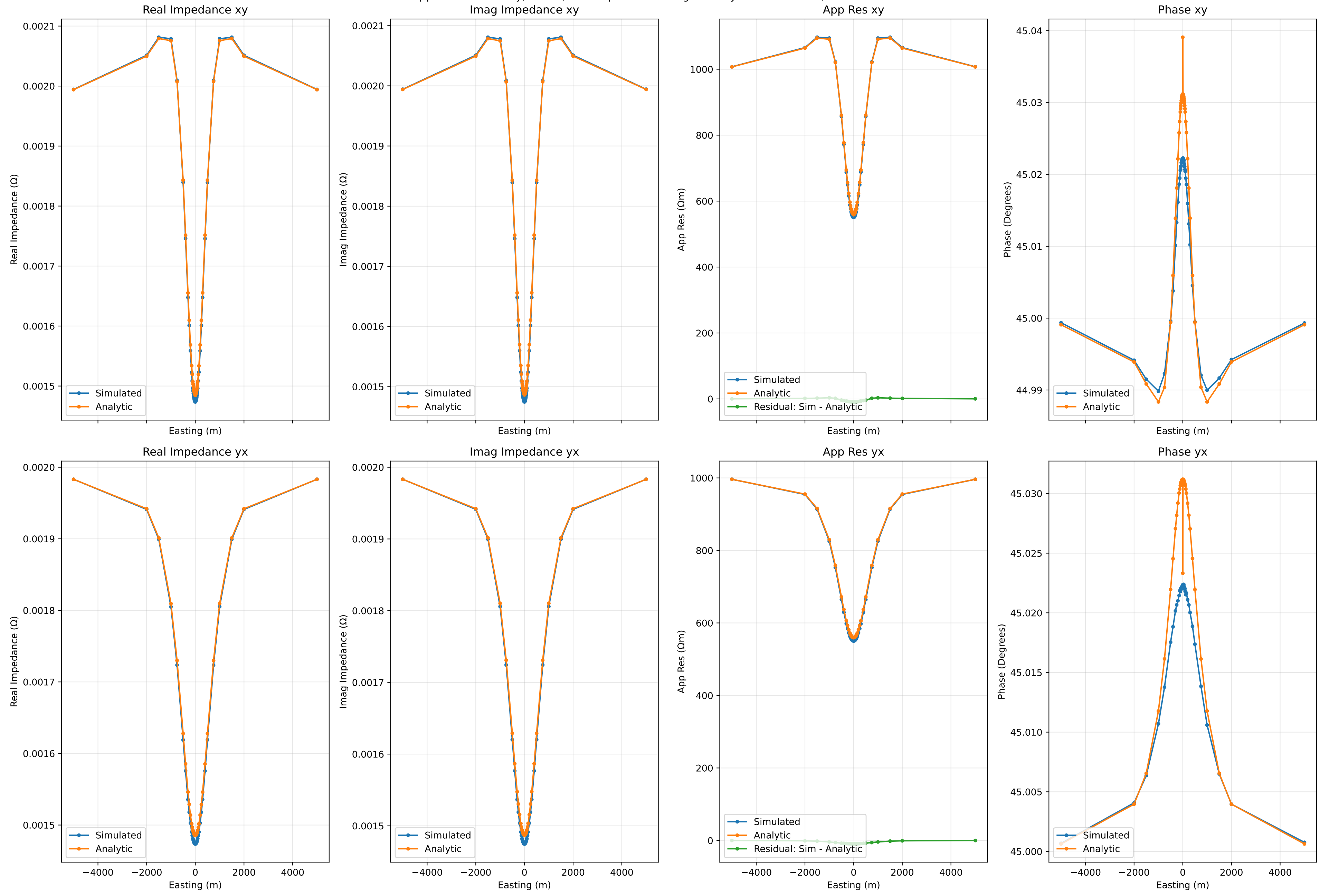
Apparent Resistivity, Phase, and Impedance along Cut at y=0 for 0.001Hz, Run Number 42
