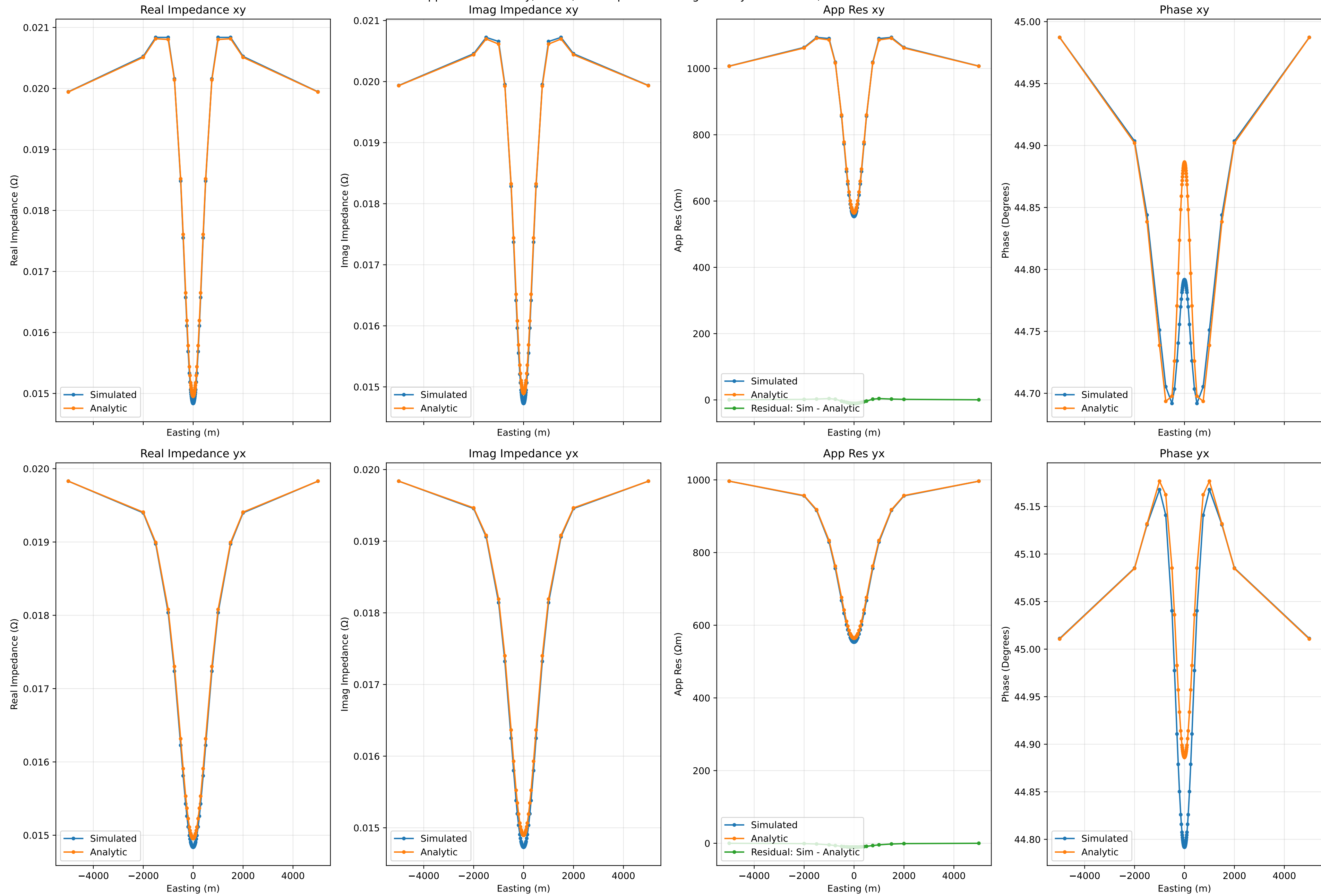
Apparent Resistivity, Phase, and Impedance along Cut at y=0 for 0.1Hz, Run Number 41
