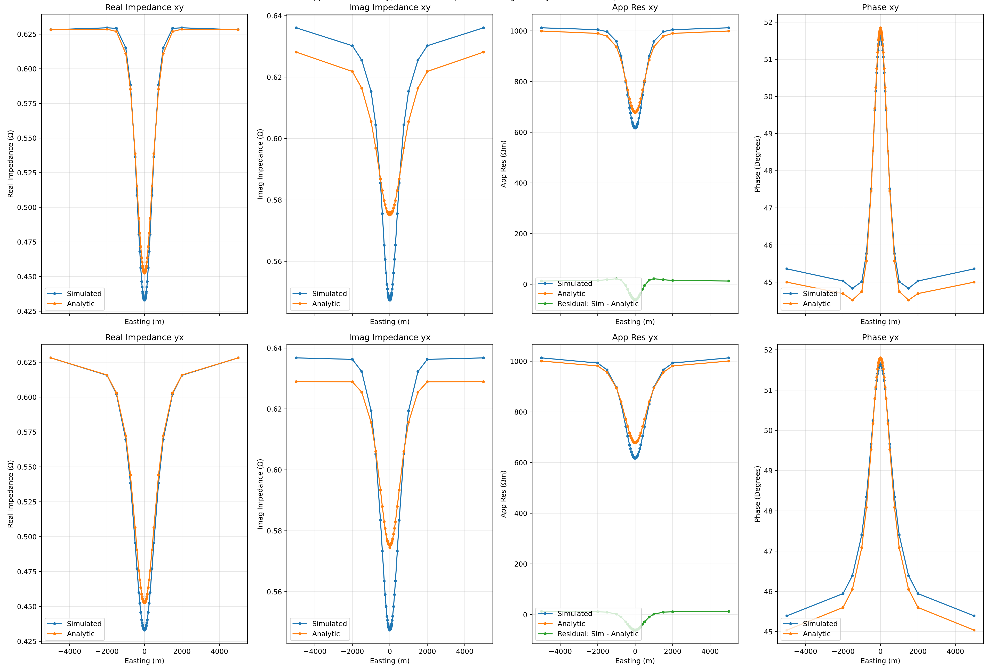
Apparent Resistivity, Phase, and Impedance along Cut at y=0 for 100.0Hz, Run Number 45
