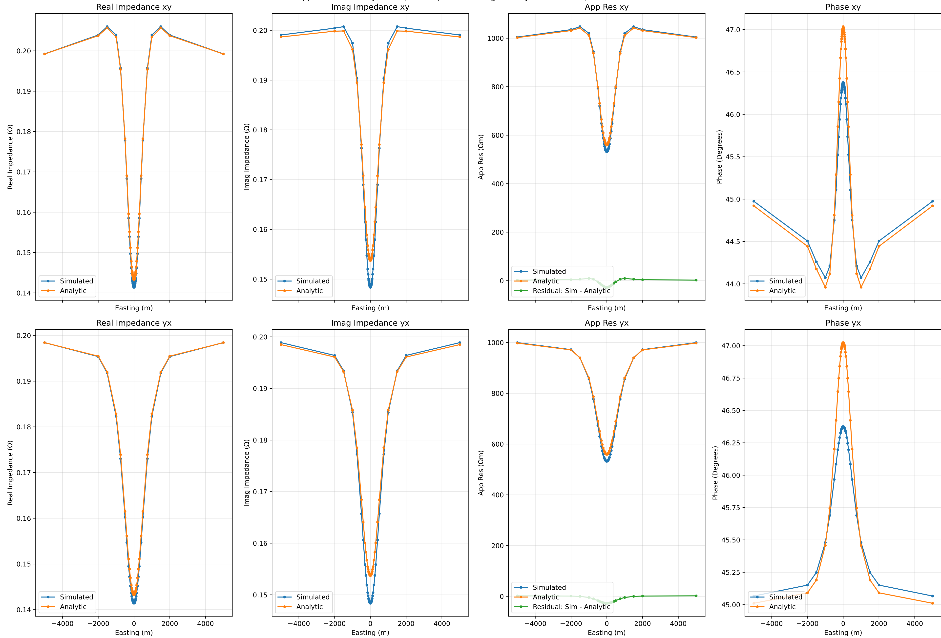
Apparent Resistivity, Phase, and Impedance along Cut at y=0 for 10.0Hz, Run Number 44
