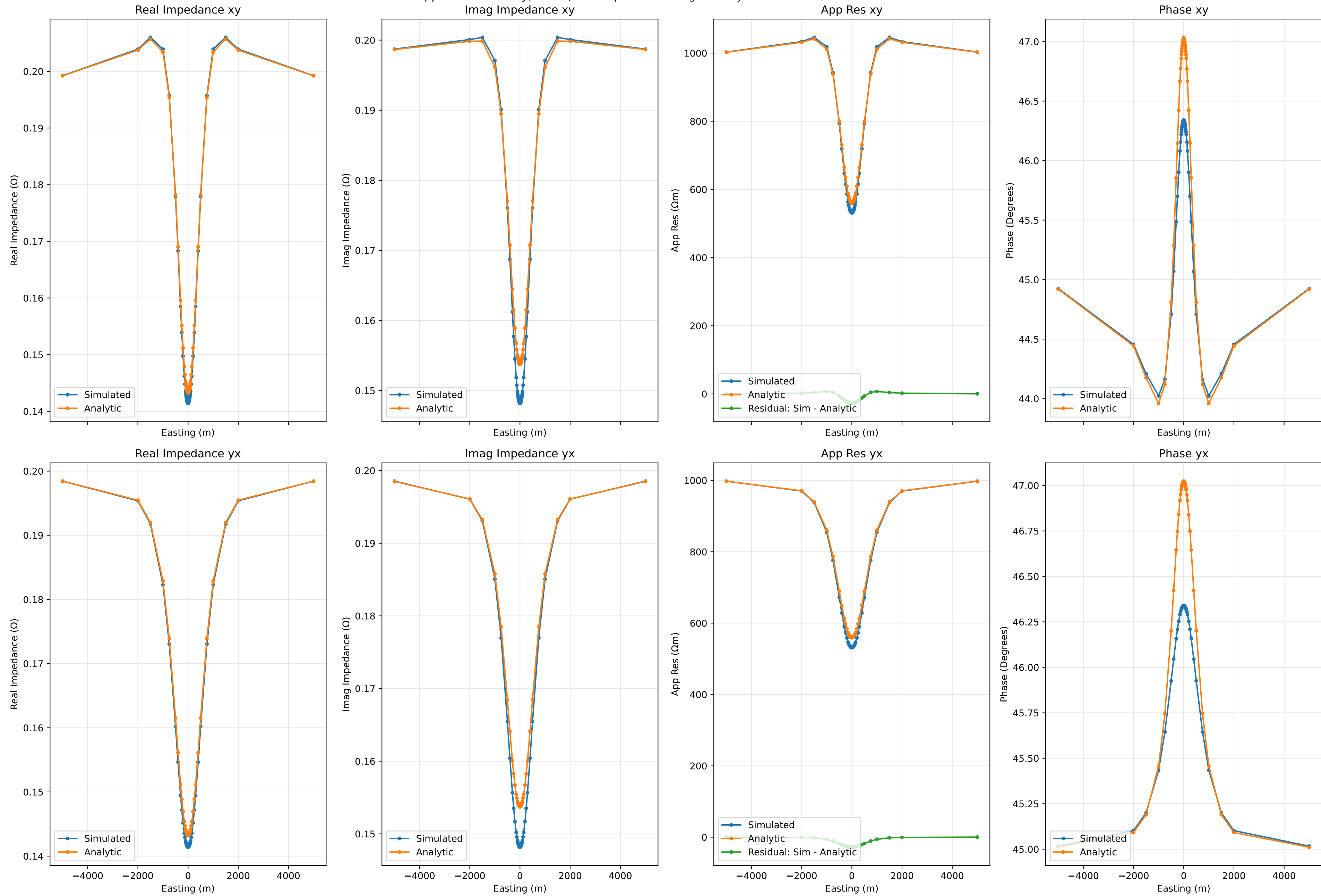
Apparent Resistivity, Phase, and Impedance along Cut at y=0 for 10.0Hz, Run Number 41
