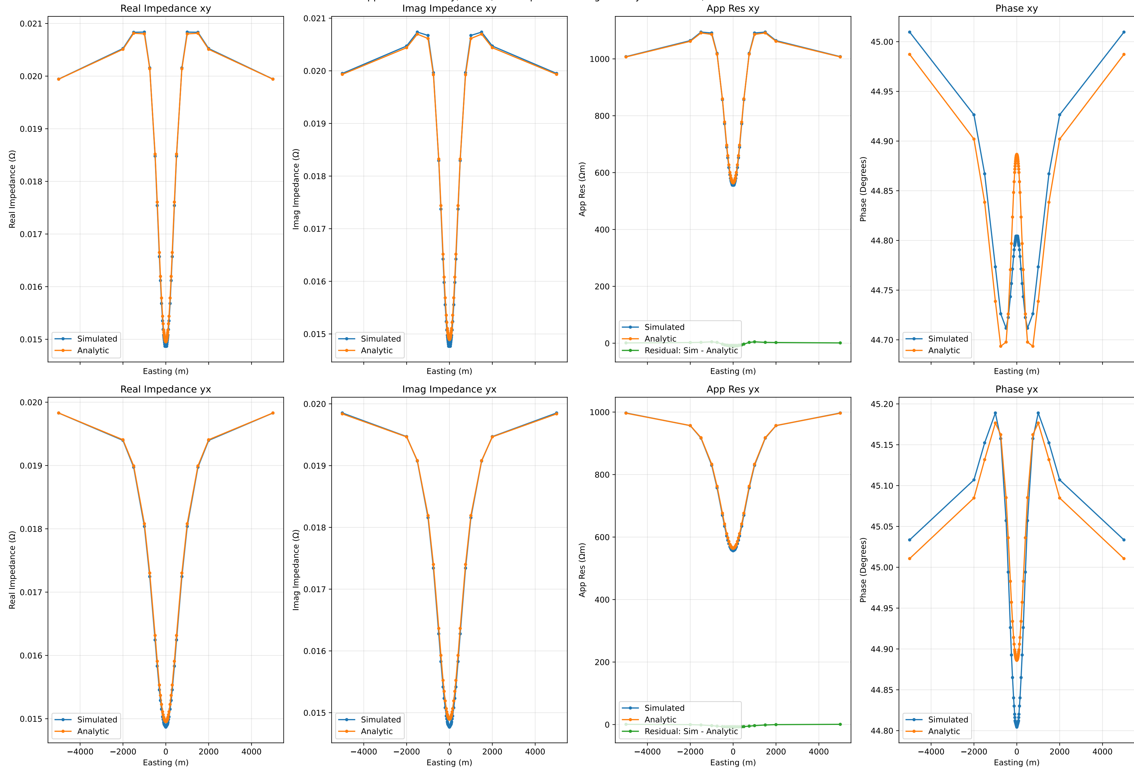
Apparent Resistivity, Phase, and Impedance along Cut at y=0 for 0.1Hz, Run Number 46
