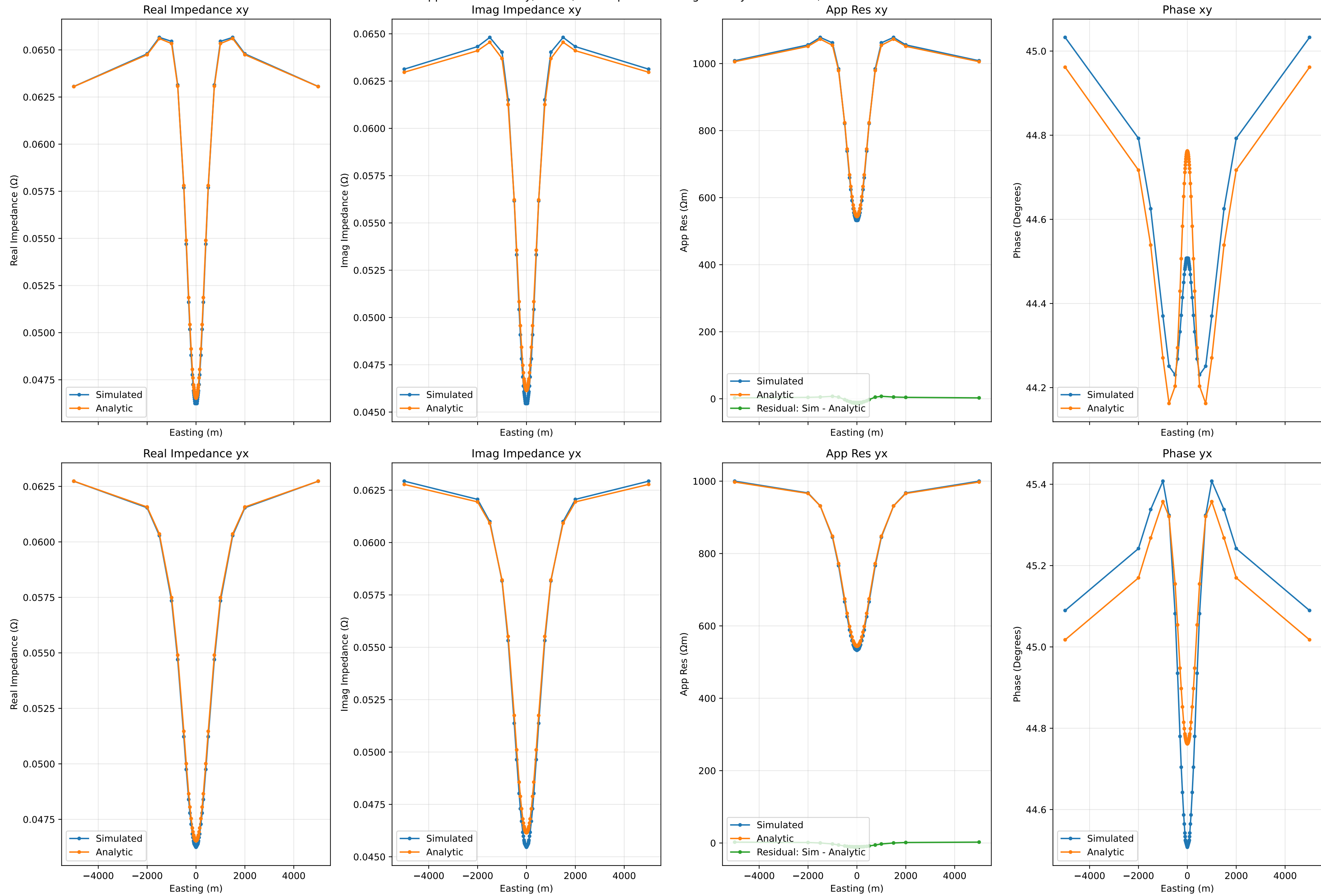
Apparent Resistivity, Phase, and Impedance along Cut at y=0 for 1.0Hz, Run Number 46
