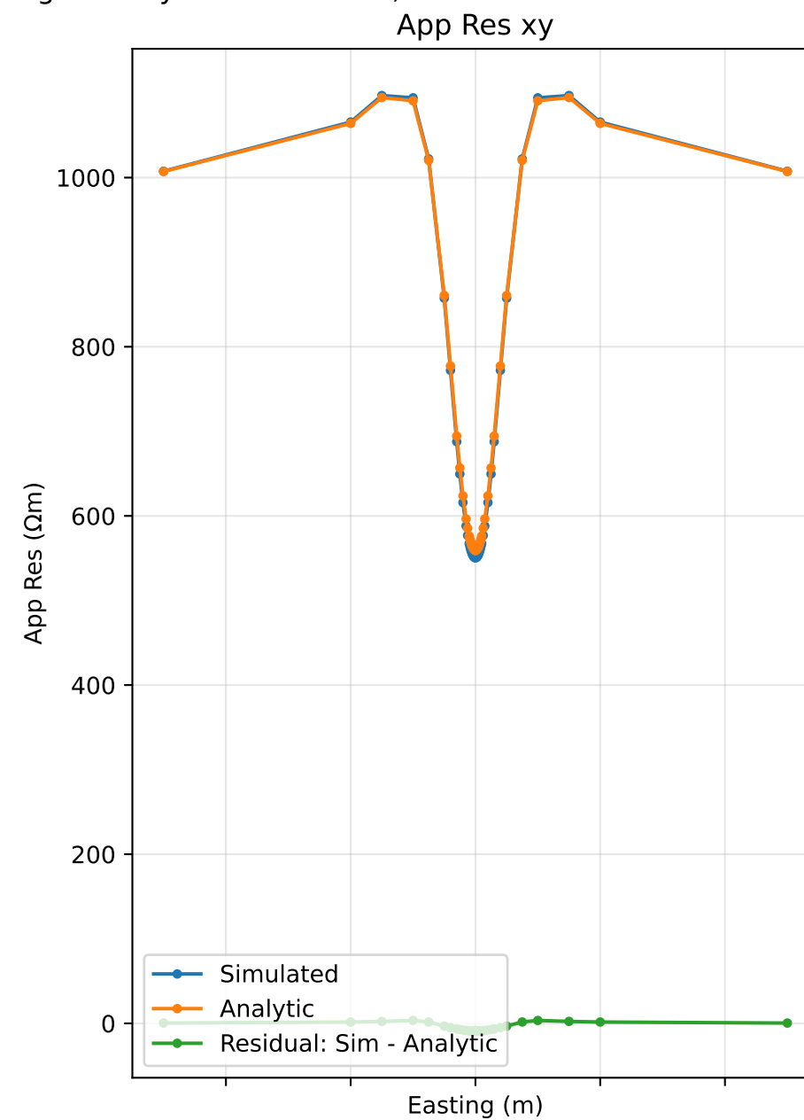
Apparent Resistivity, Phase, and Impedance along Cut at y=0 for 0.001Hz, Run Number 43
