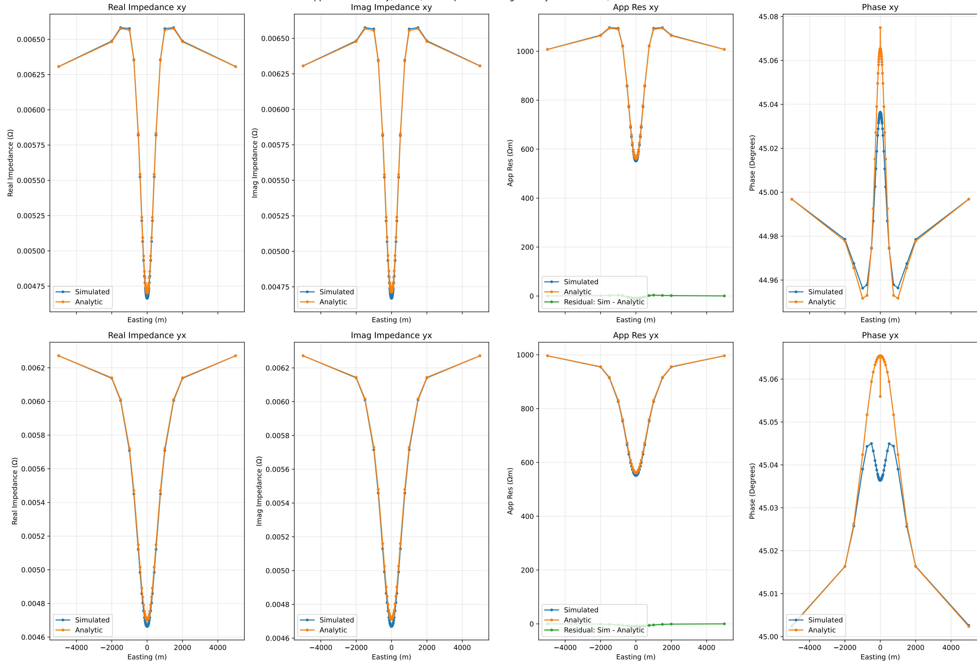
Apparent Resistivity, Phase, and Impedance along Cut at y=0 for 0.01Hz, Run Number 41
