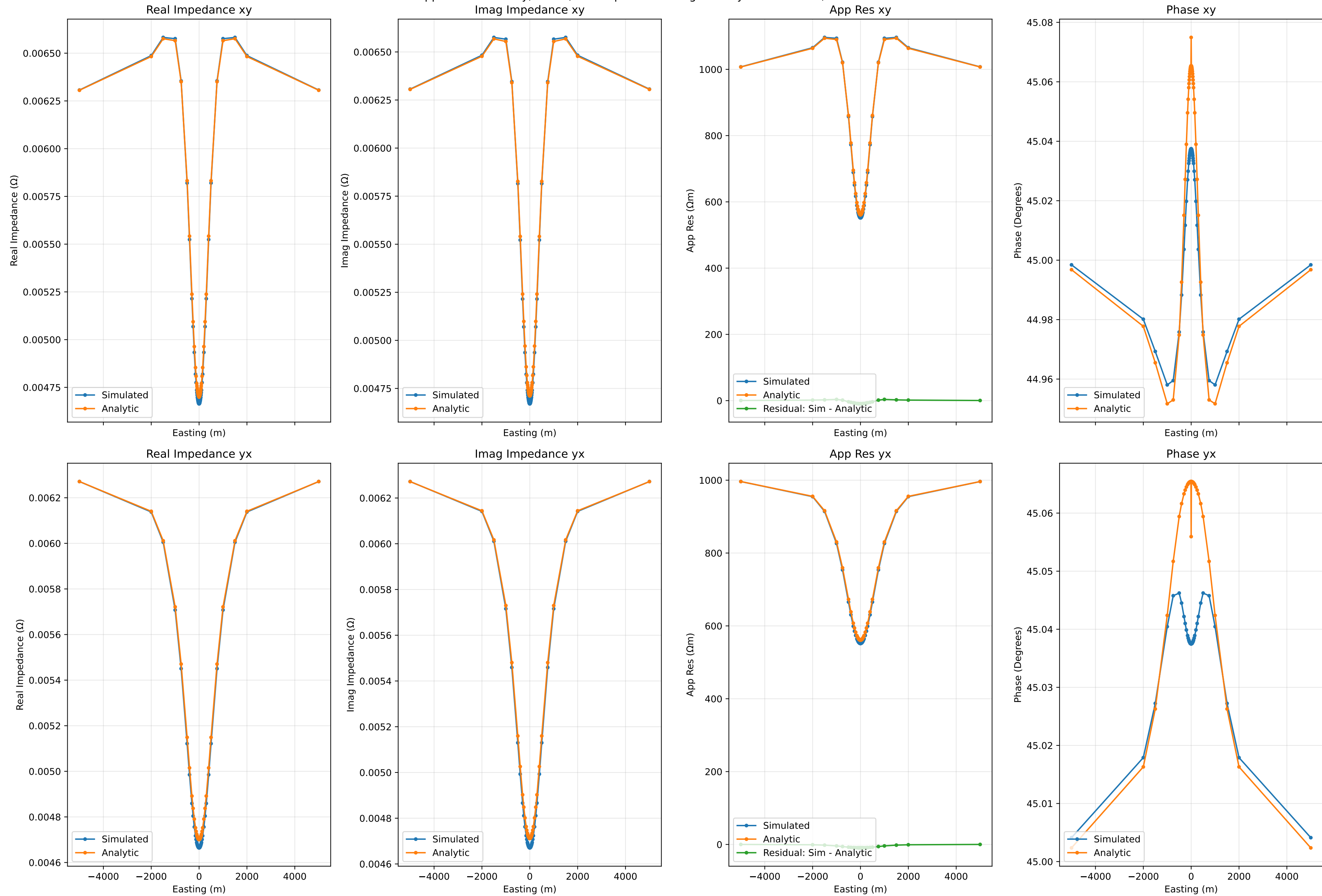
Apparent Resistivity, Phase, and Impedance along Cut at y=0 for 0.01Hz, Run Number 44
