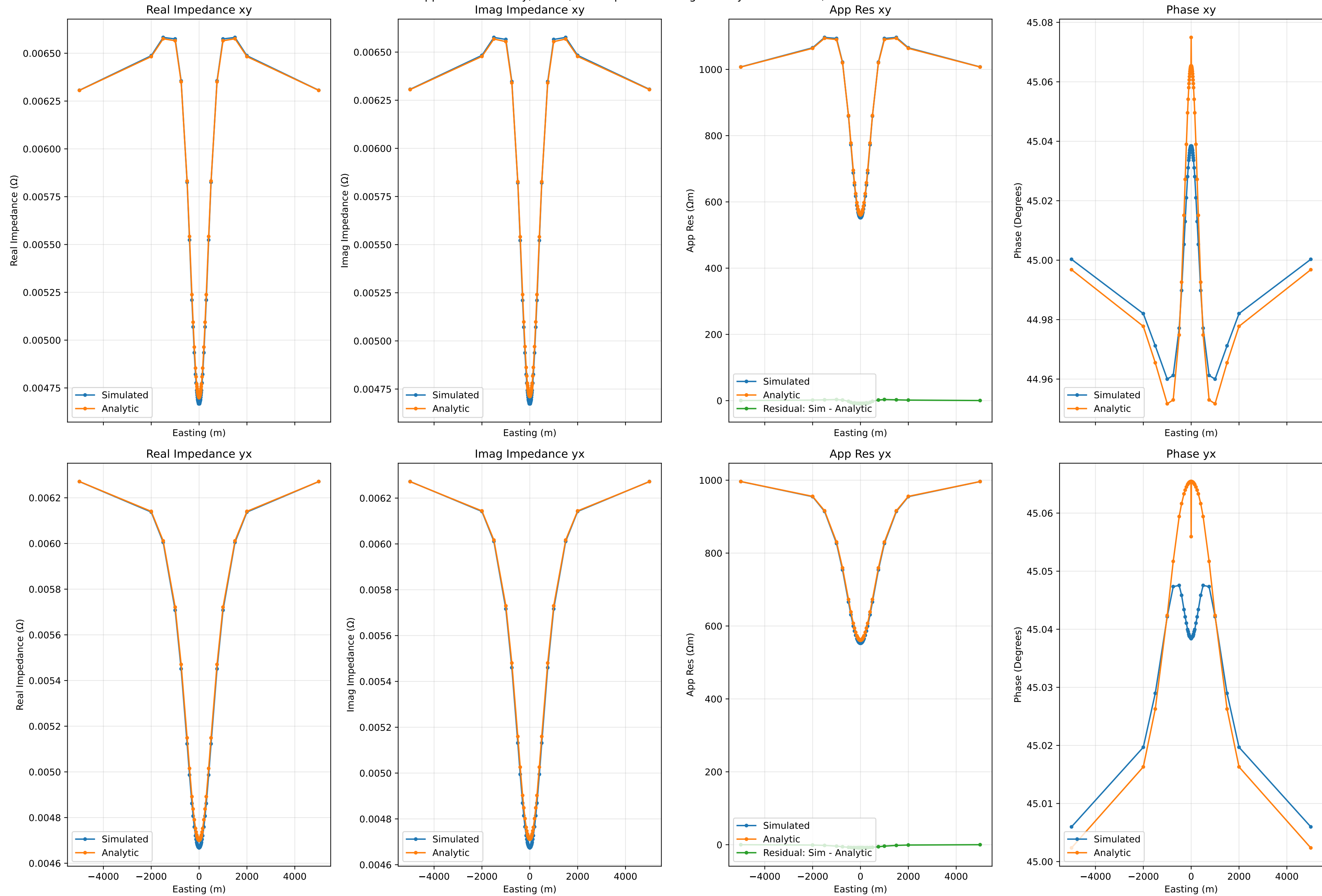
Apparent Resistivity, Phase, and Impedance along Cut at y=0 for 0.01Hz, Run Number 45
