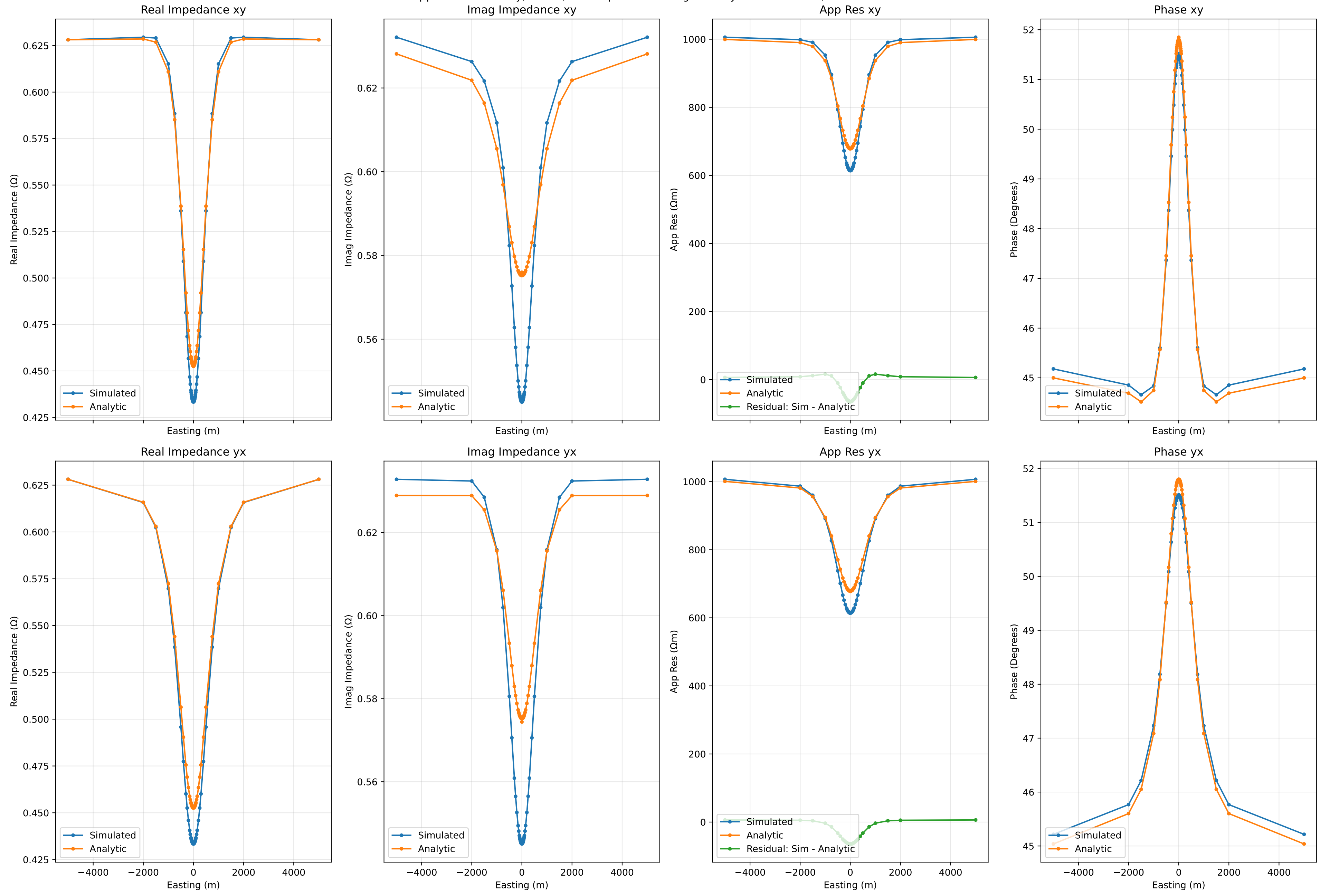
Apparent Resistivity, Phase, and Impedance along Cut at y=0 for 100.0Hz, Run Number 44
