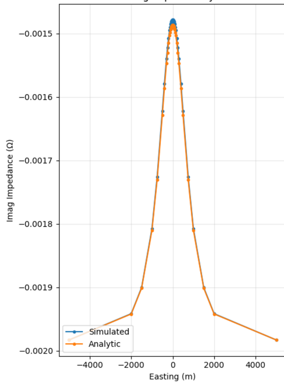
Imag Impedance yx
