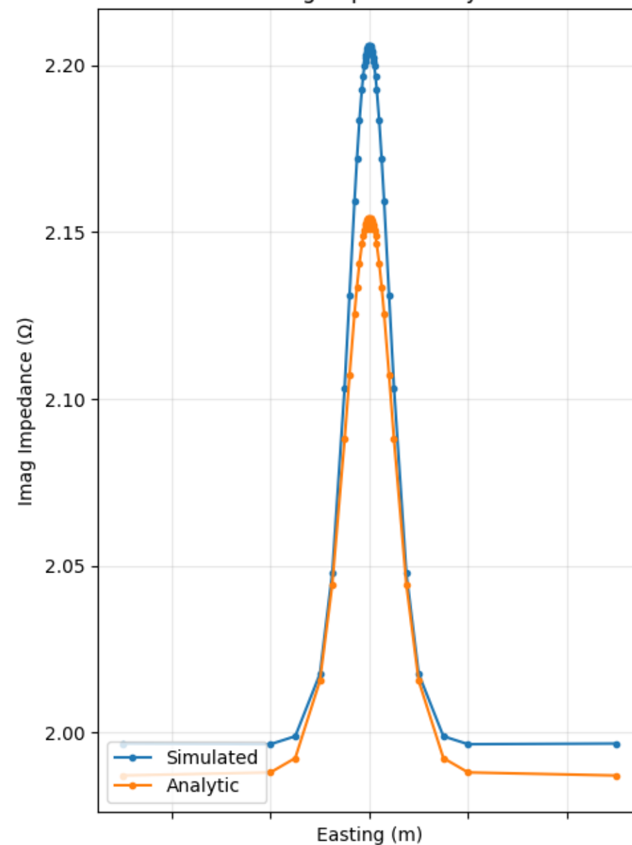
Apparent Resistivity, Phase, and Impedance along Cut at y=0 for 1000.0Hz Imag Impedance xy
