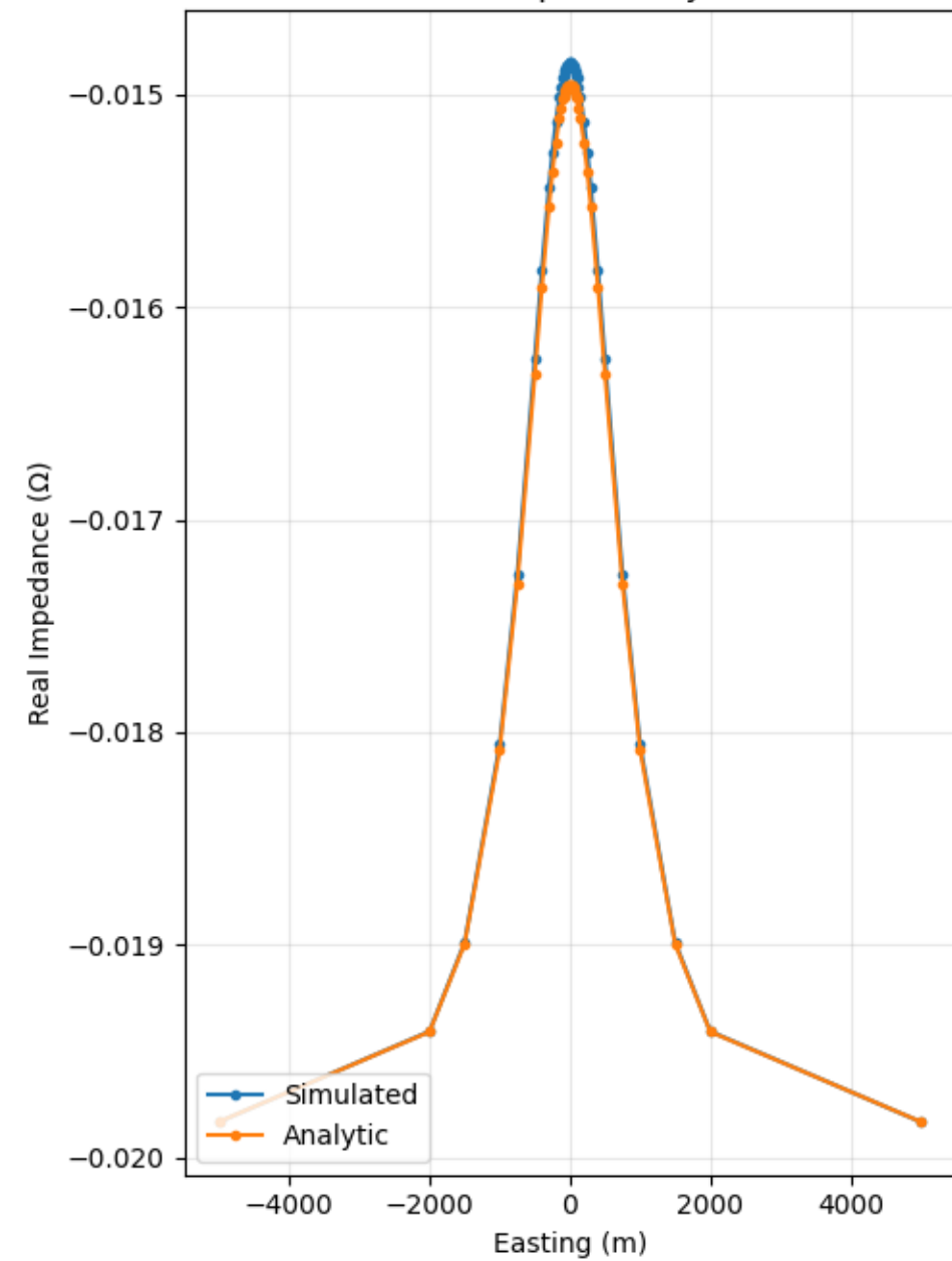
Real Impedance yx
