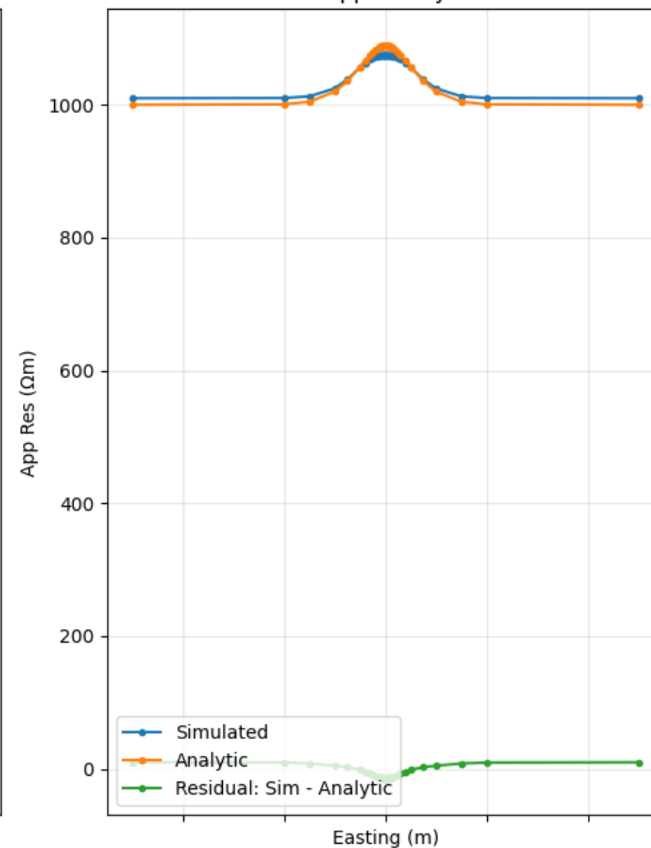
Apparent Resistivity, Phase, and Impedance along Cut at y=0 for 1000.0Hz Imag Impedance xy App Res xy
