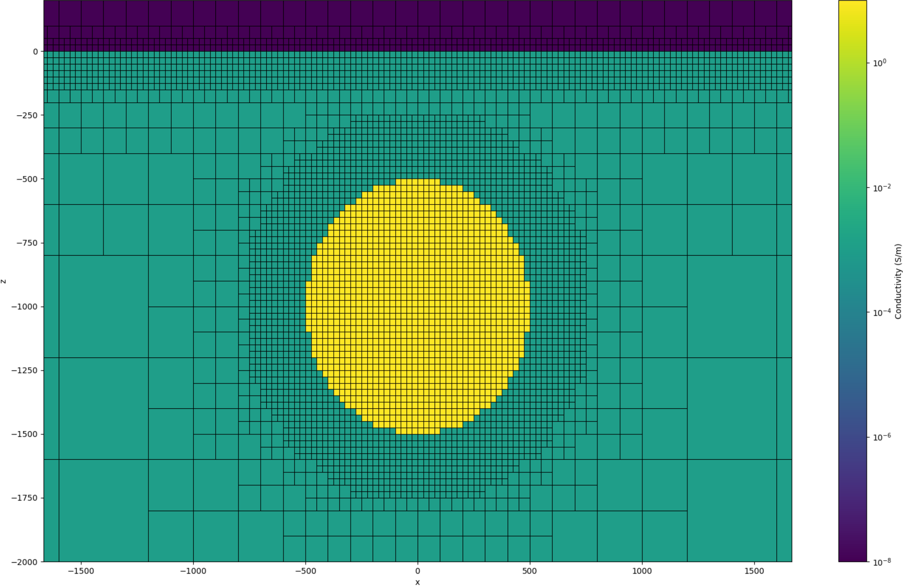
Conductivity Model Cross Section at y=0, 1586796 cells
