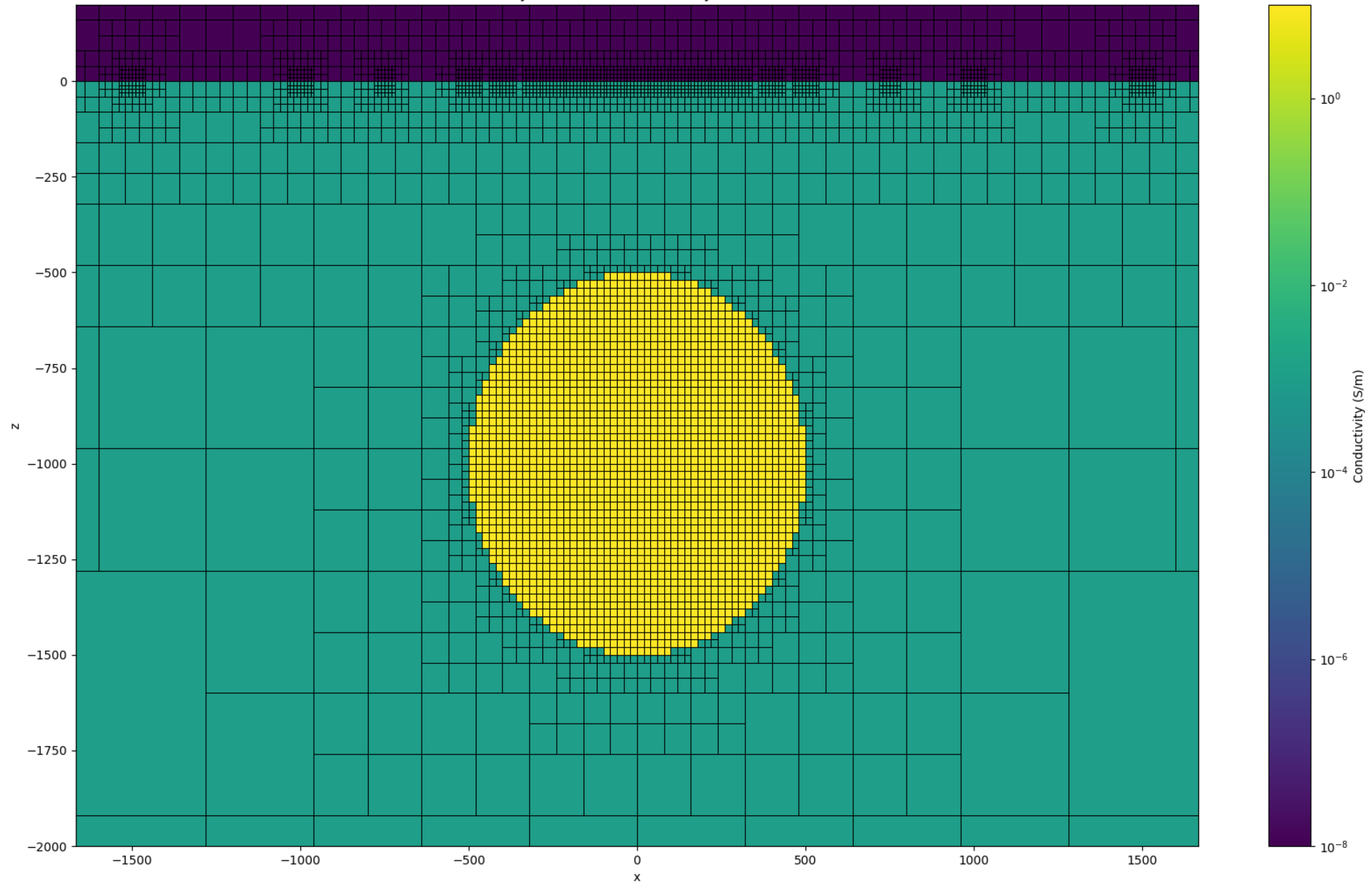
Conductivity Model Cross Section at y=0, 788292 cells
