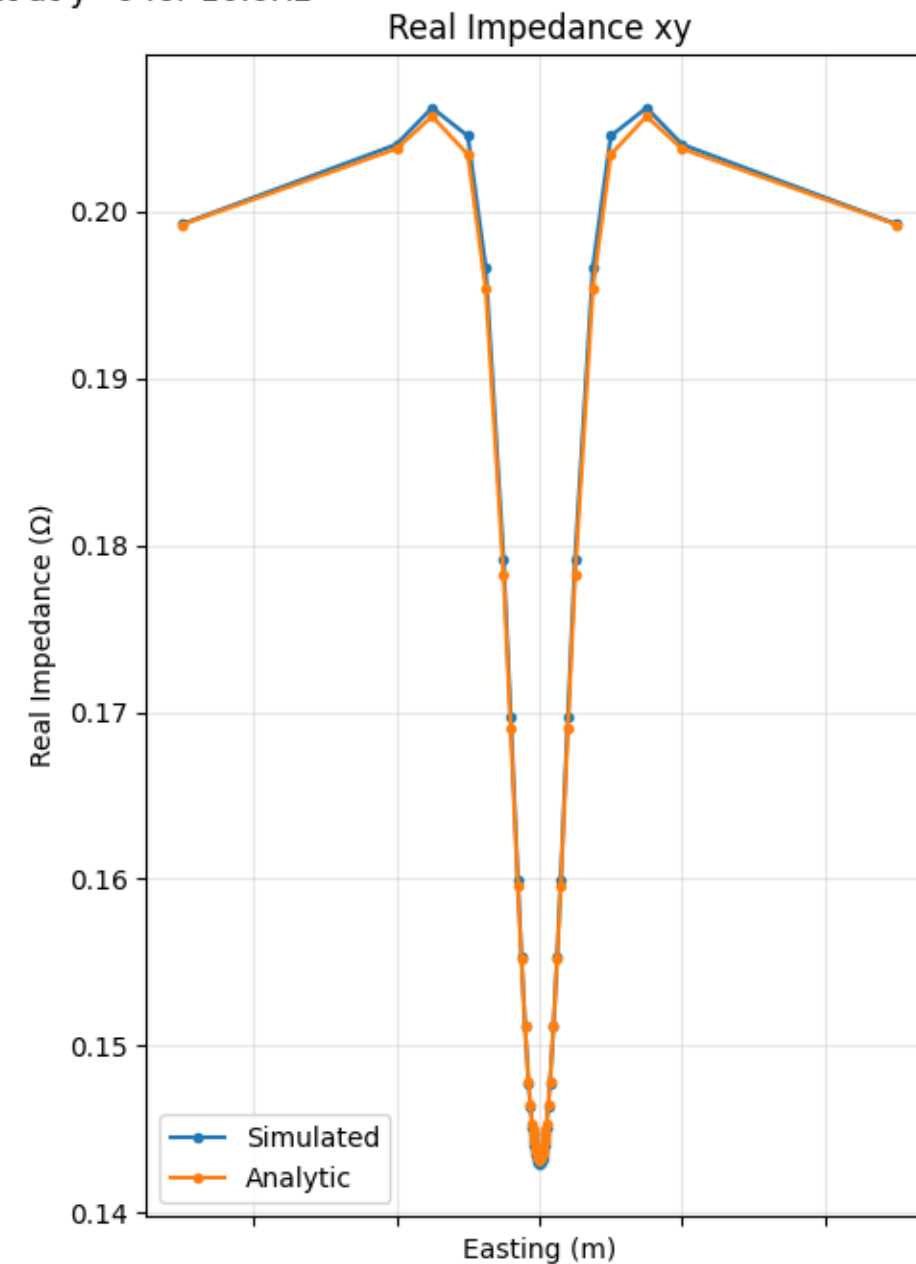
Impedance along Cut at y=0 for 10.0Hz
