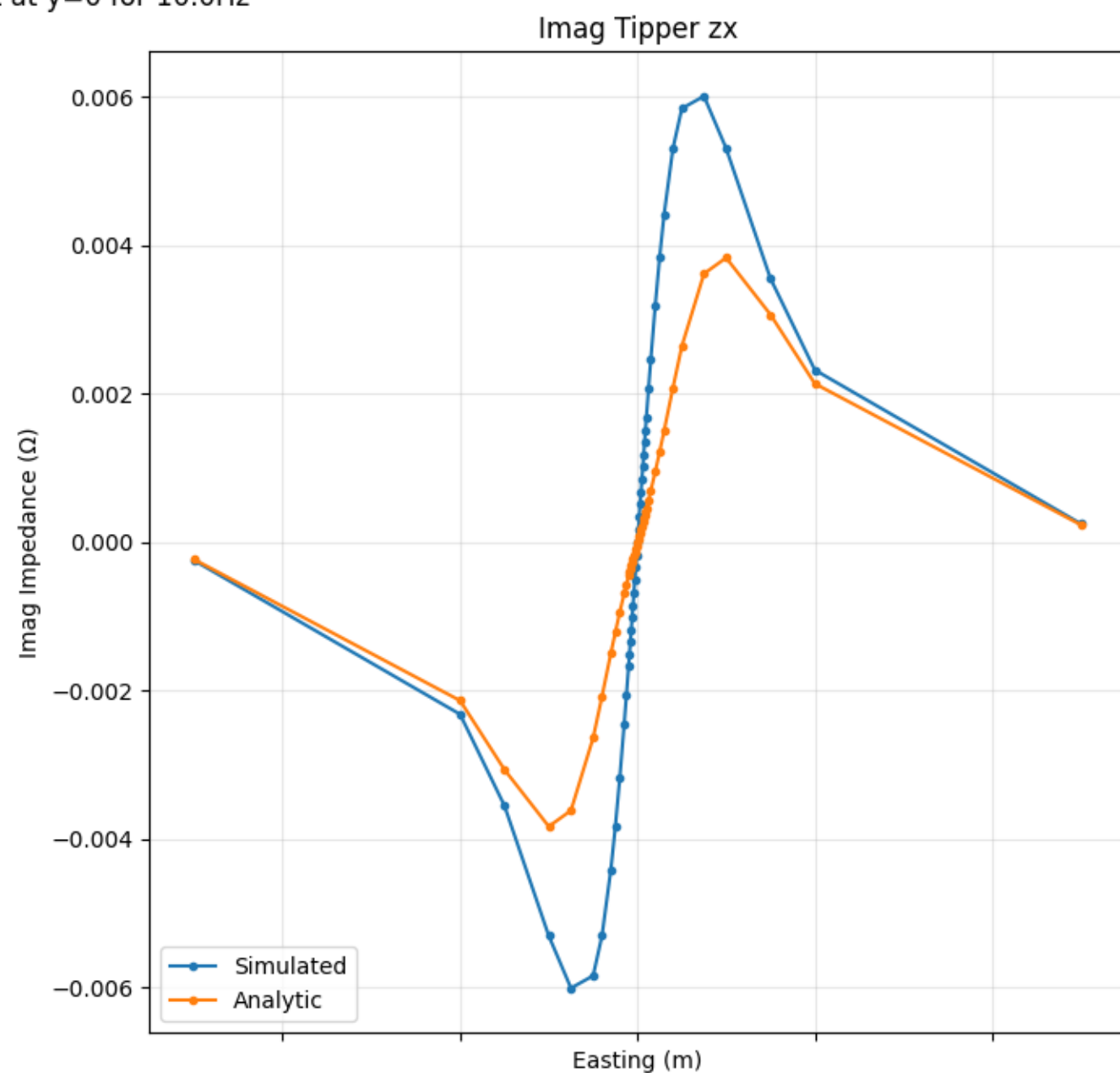
Tipper along Cut at y=0 for 10.0Hz
