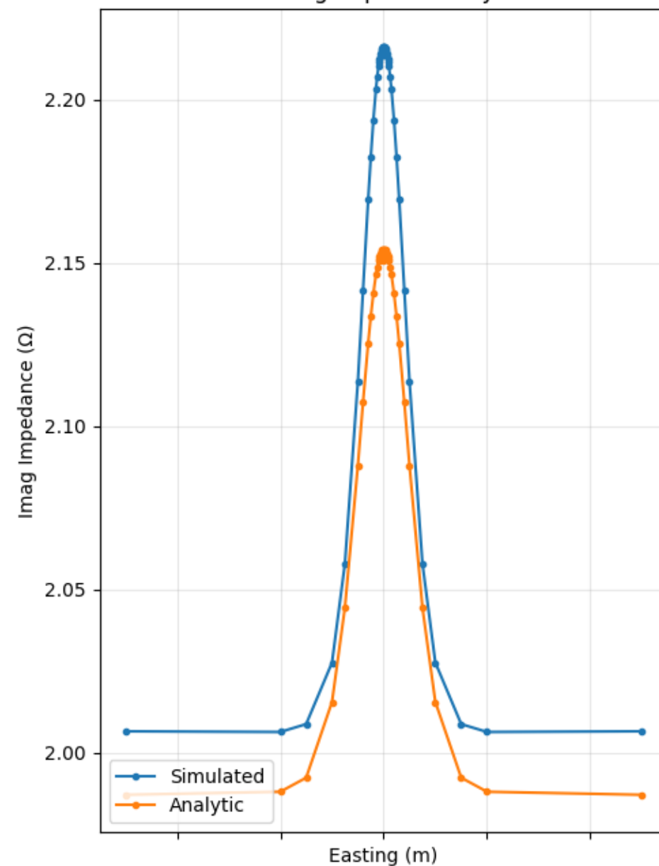
Apparent Resistivity, Phase, and Impedance along Cut at y=0 for 1000.0Hz
