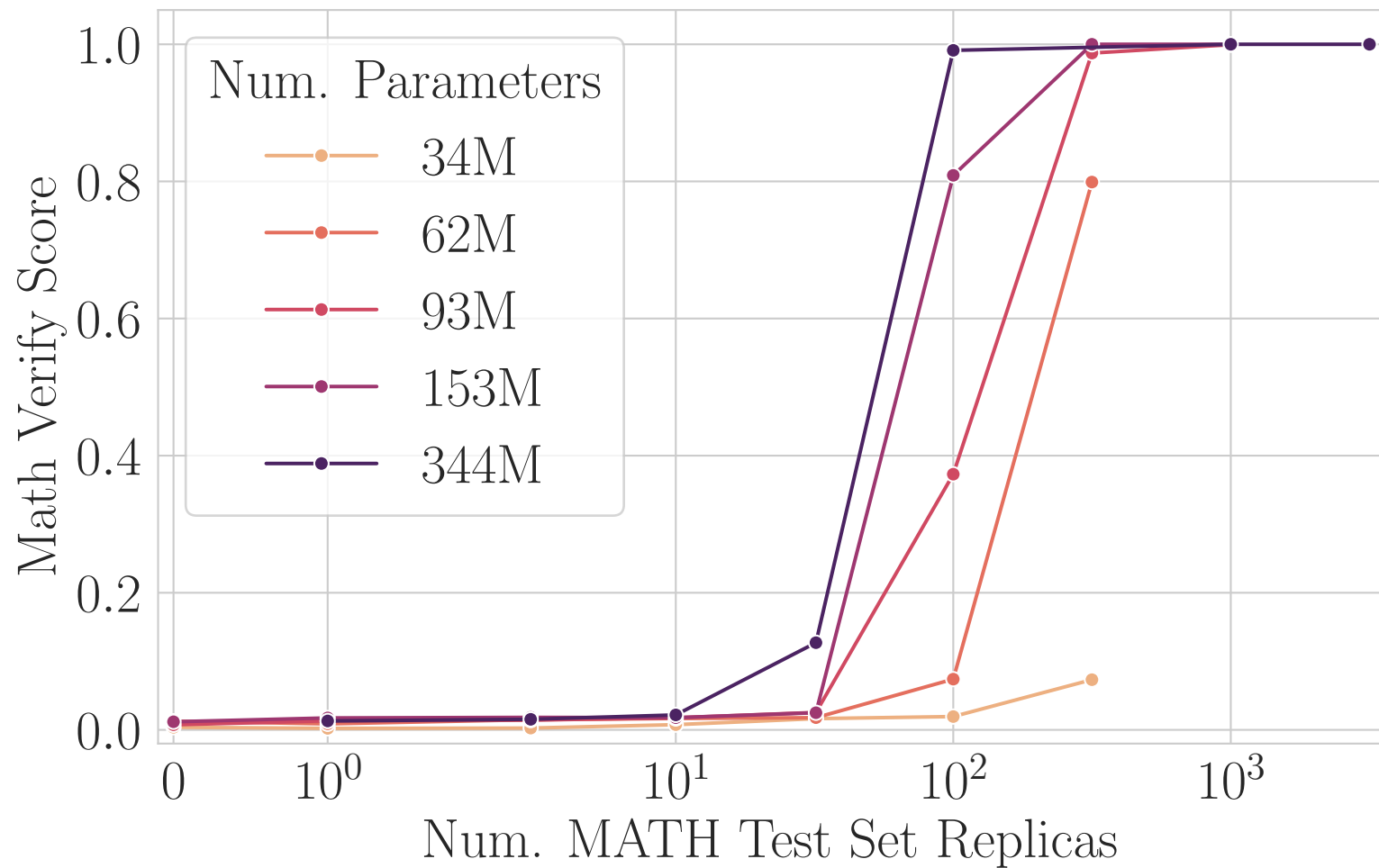
0-shot
