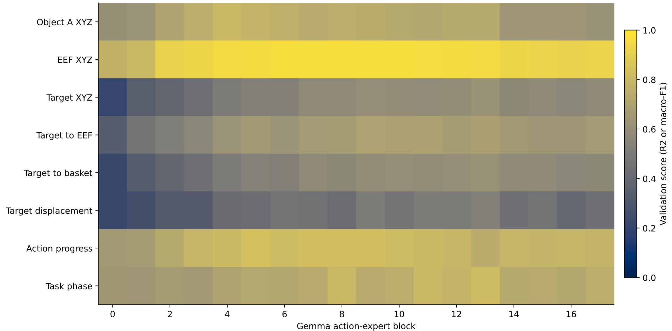
pi0.5 action-token mean world-state atlas at t=1.0
