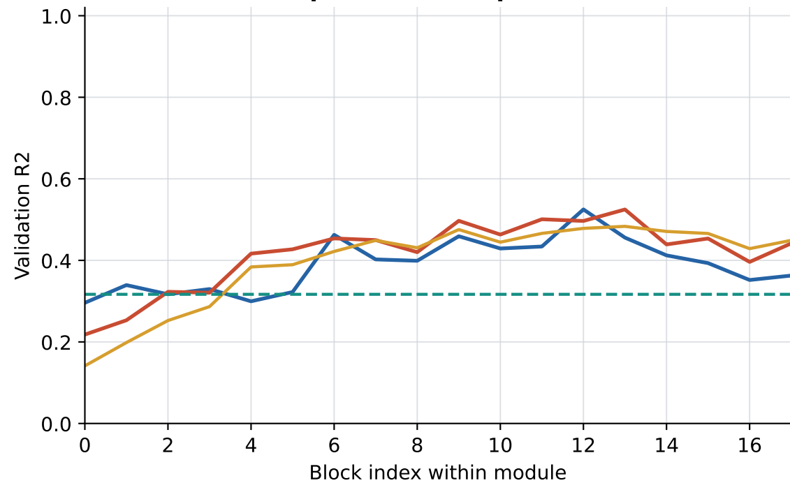
Prompt-relative displacement
