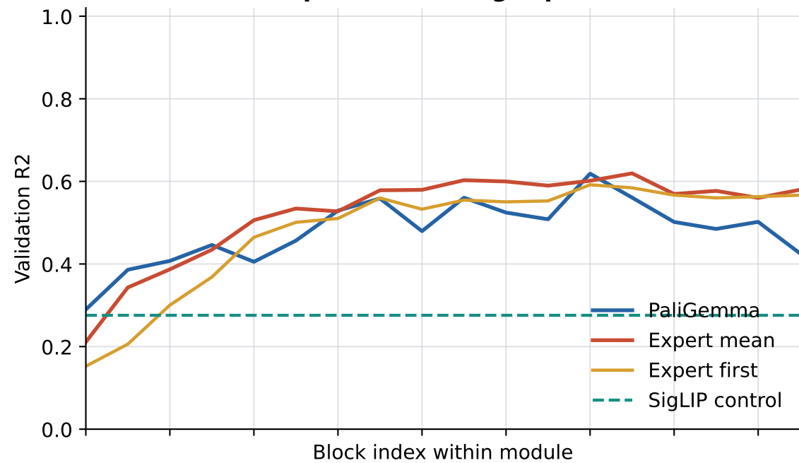
Prompt-relative displacement
