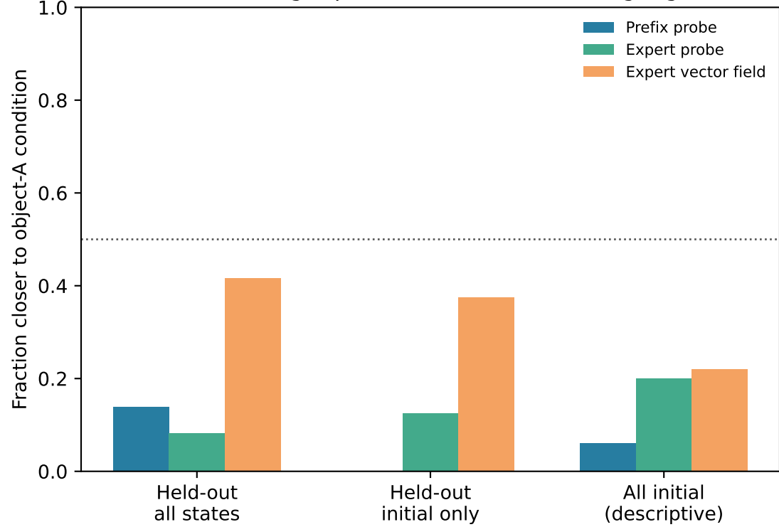
Default target preference under null language
