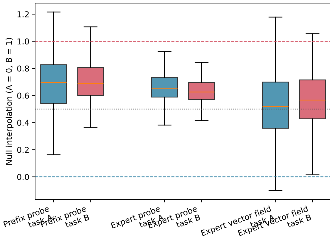
Where the target-unspecified prompt lands
