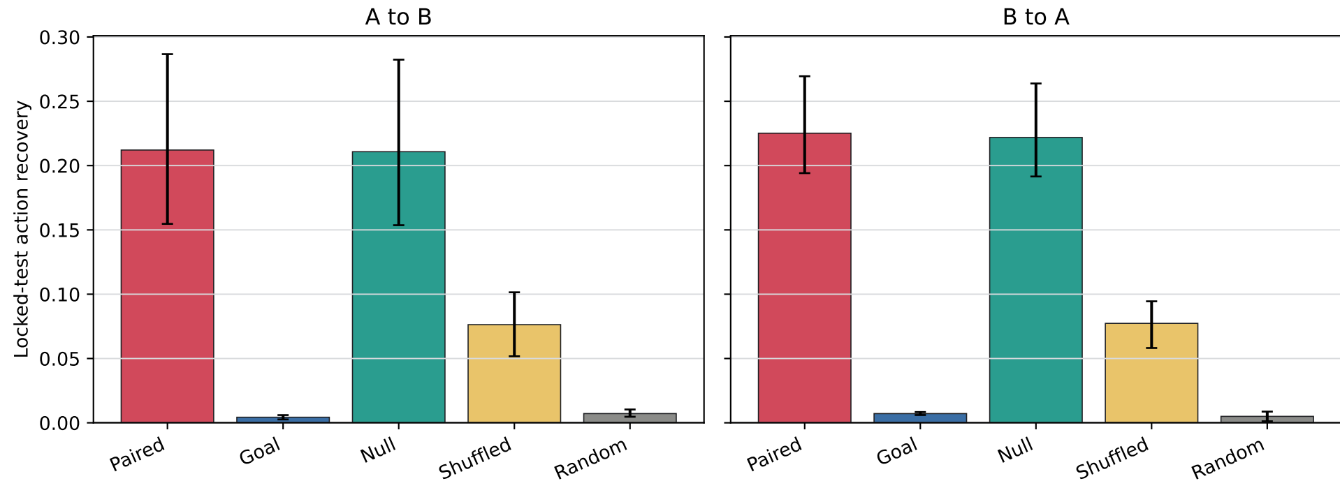
Block 13 semantic and matched controls (95% episode-bootstrap CI)
