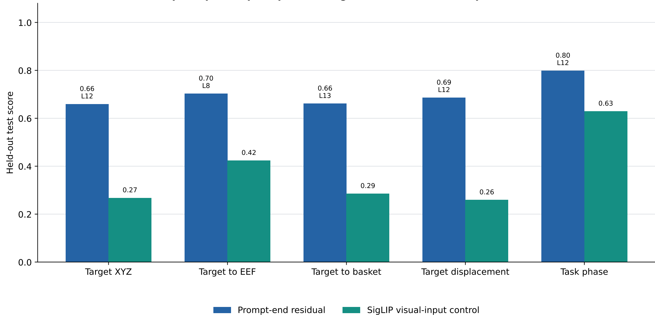
pi0.5 paired-prompt decoding on held-out LIBERO episodes
