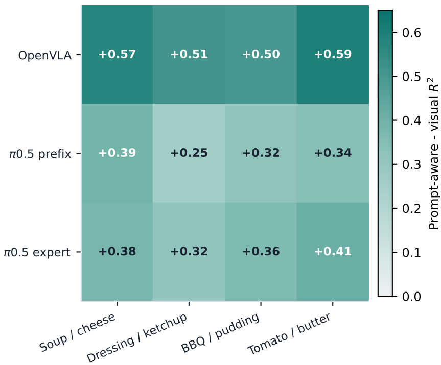
c Pooled gain is positive for every pair
