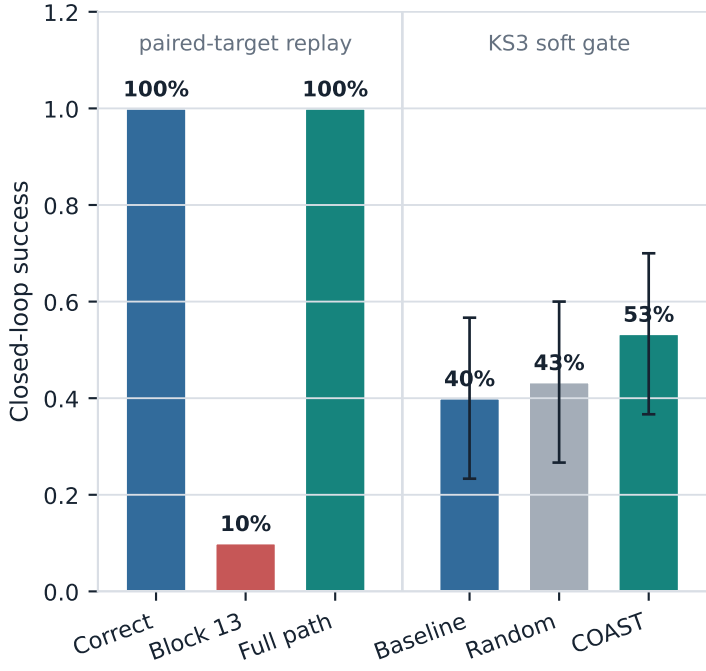
f Causal use depends on pathway-compatible operators
