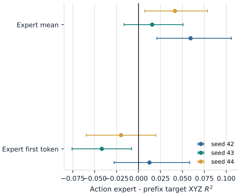
e Propagation is real; extra decodability is modest
