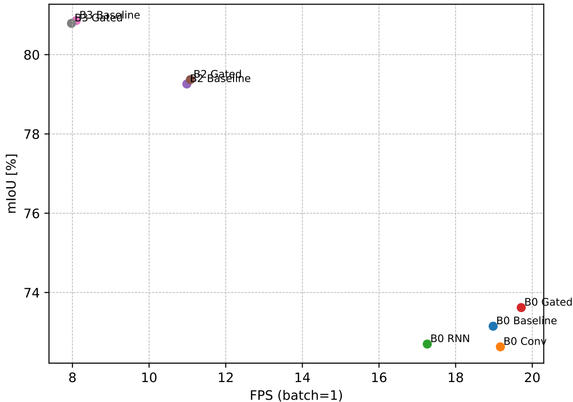
Trade-off: mIoU vs FPS (160k)
