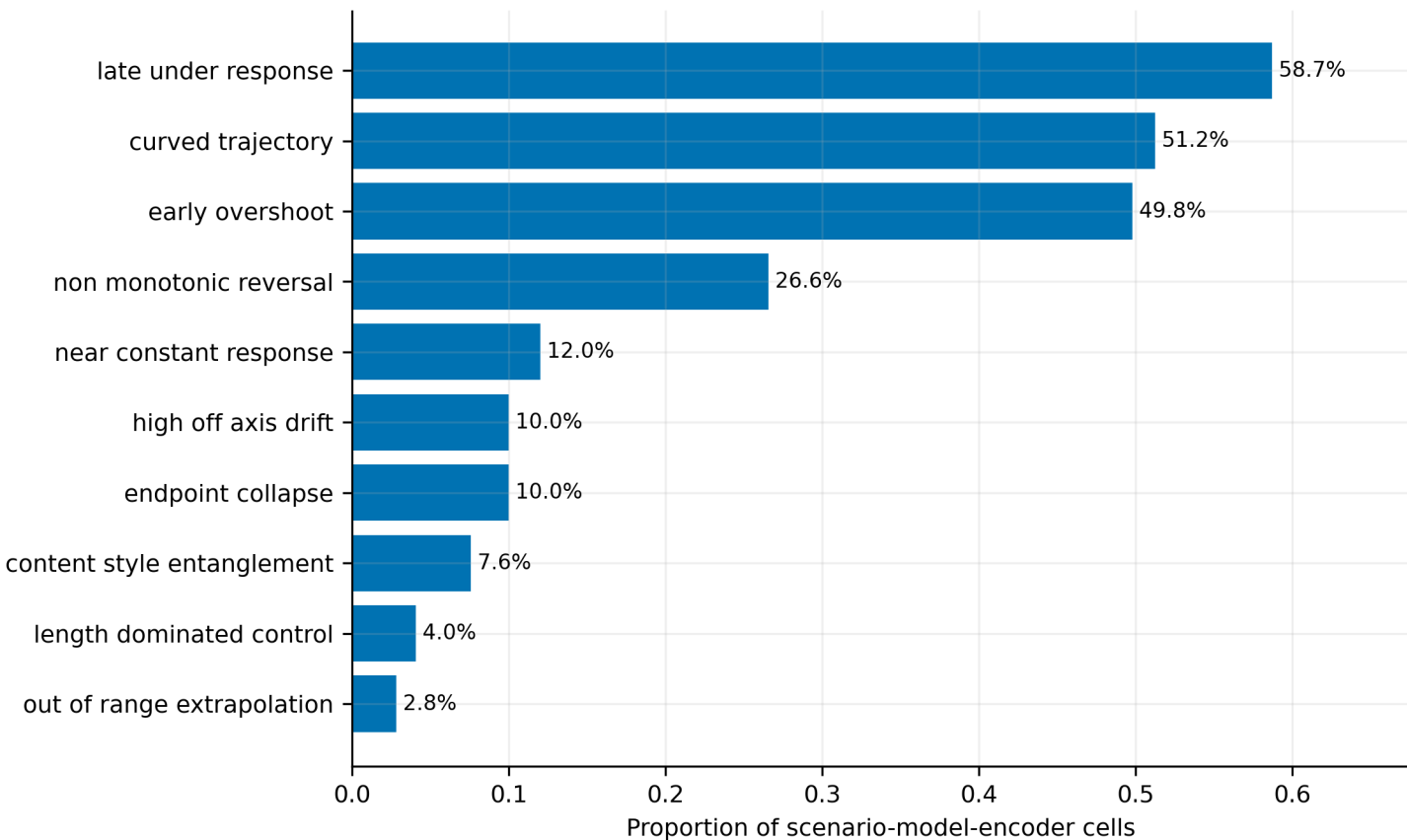
Prespecified control failure taxonomy
