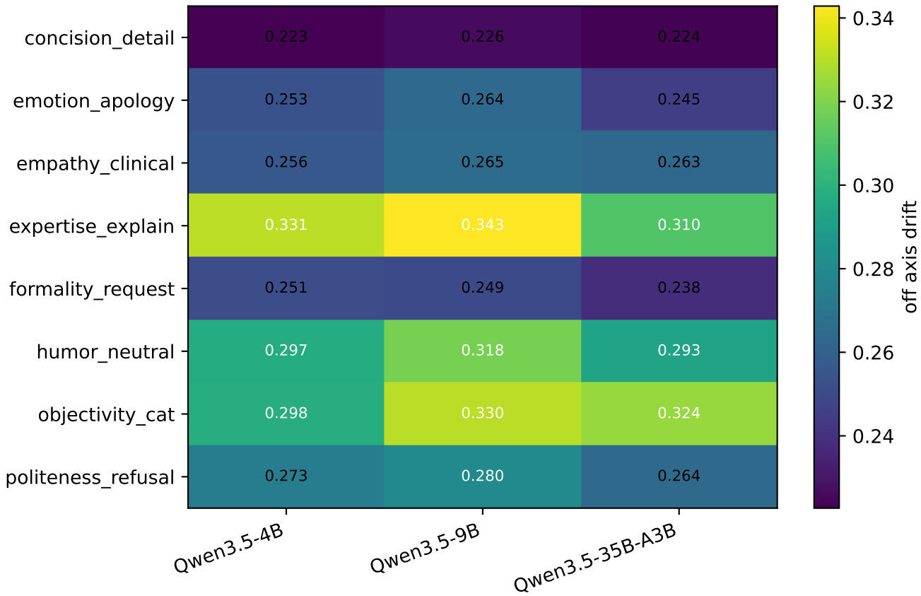
Off-Axis Drift by Axis (bge-m3)
