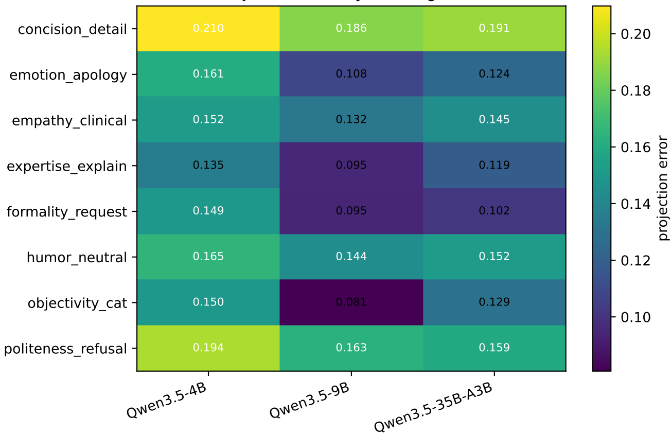
Projection MAE by Axis (bge-m3)
