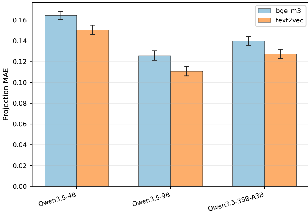
Projection MAE with Scenario-bootstrap 95% CI
