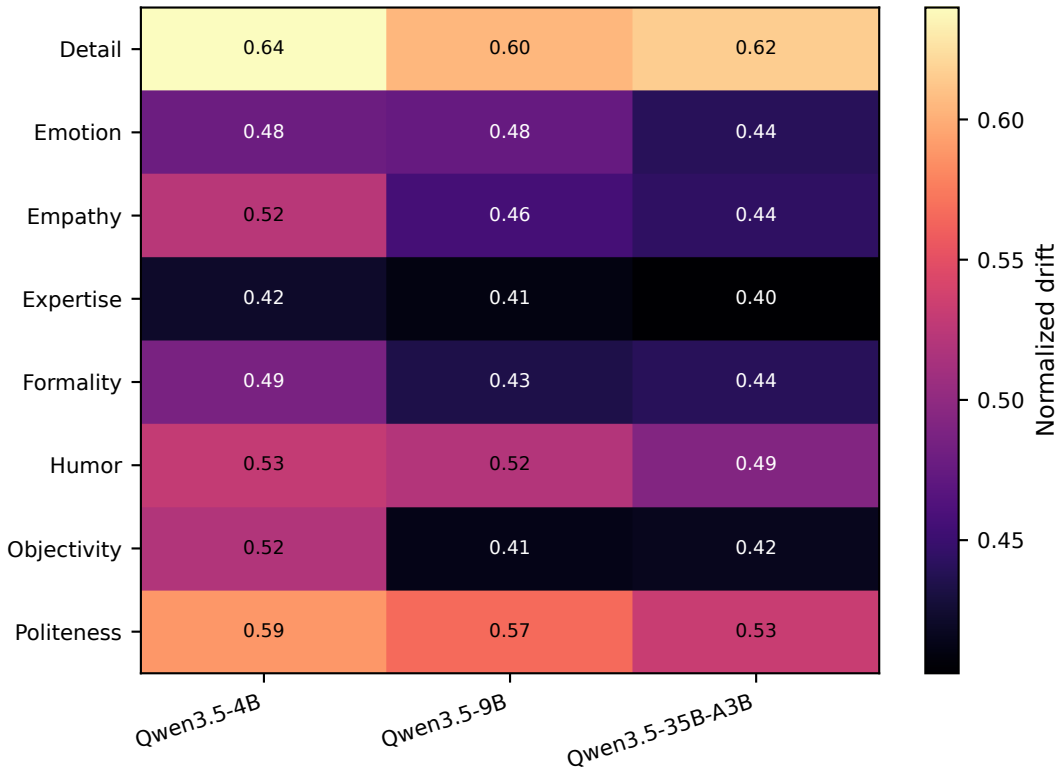
Normalized Off-axis Drift by Axis
