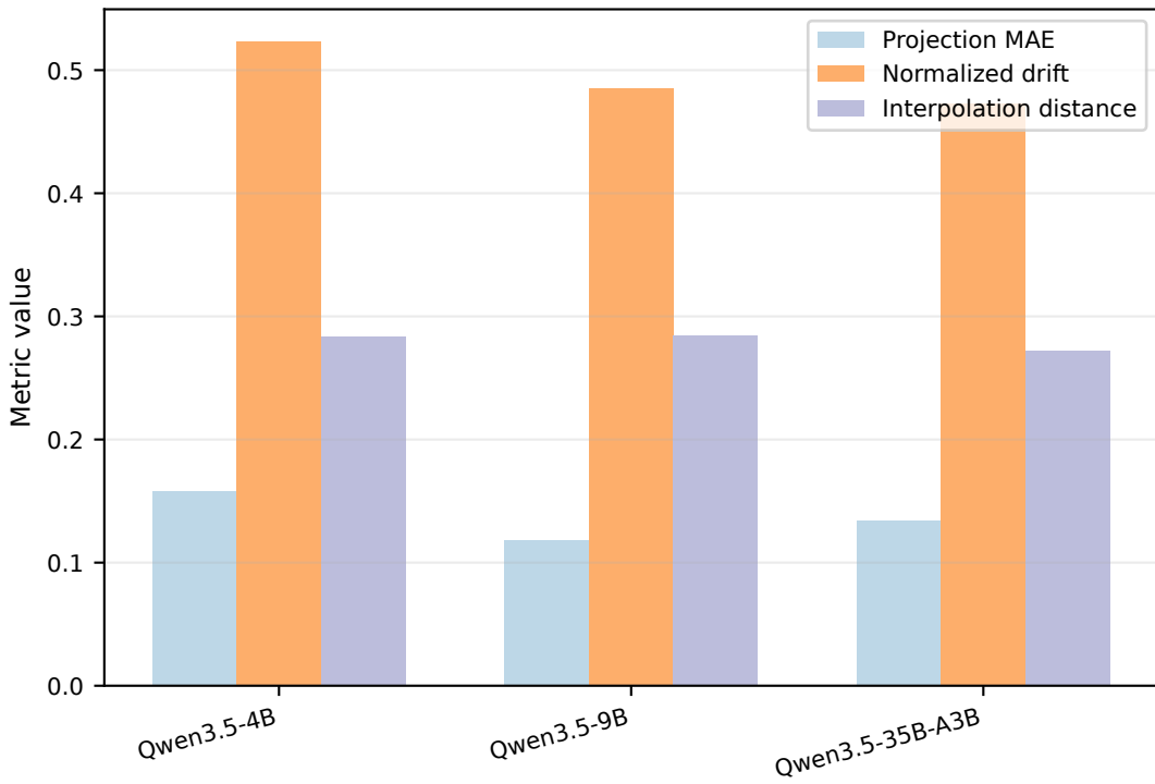
Geometry Decomposition by Model
