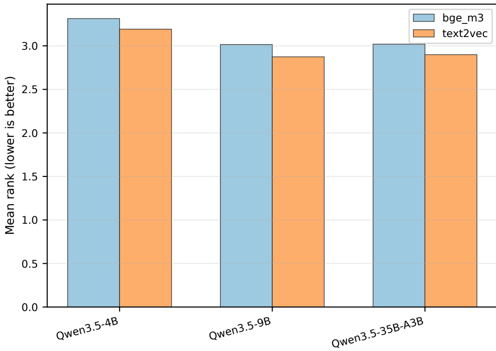
Nearest-neighbor Mean Rank
