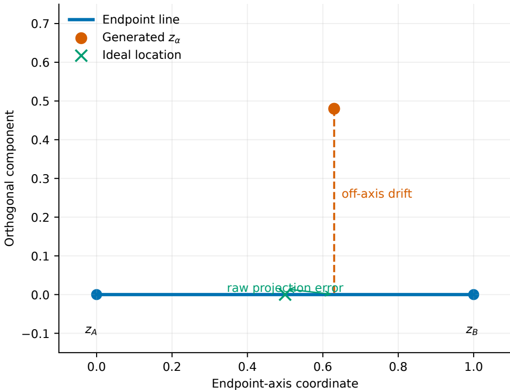
Raw projection and normalized off-axis drift
